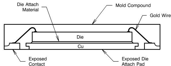
Figure 47. Internal Connection
