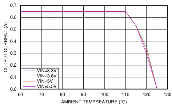
Figure 6-3. Thermal Derating V_{OUT} = 1.2\text{ V} , \theta_{JA} = 77^\circ\text{C/W}
