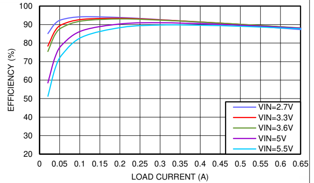
Figure 8-9. Efficiency V_{OUT} = 1.8\text{ V}
