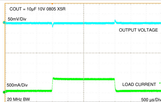
Figure 8-11. Load Transient V_{OUT} = 1.8\text{ V}
