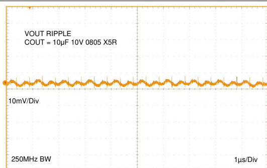
Figure 8-16. Output Ripple V_{OUT} = 2.5\text{ V}
