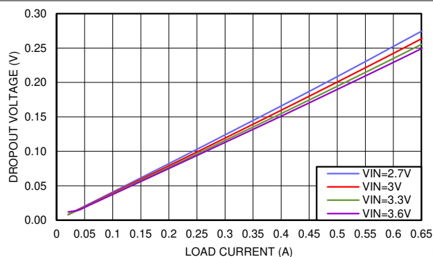
Figure 6-2. Dropout Voltage vs Load Current and Input Voltage
