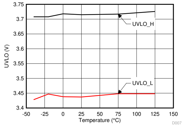
Figure 5-12. UVLO Threshold
