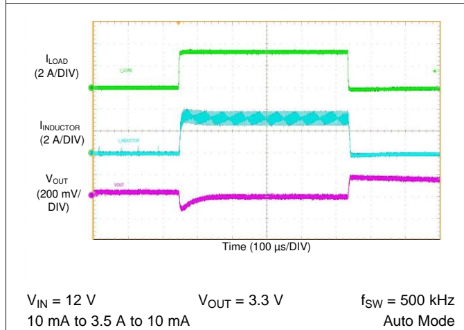
Figure 73. LM76003 Load Transient
