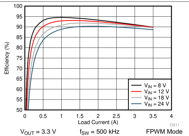
Figure 24. LM76003 Efficiency
