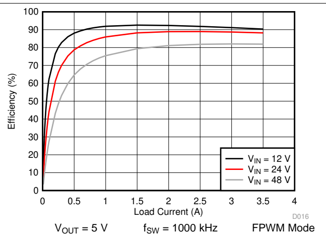
Figure 28. LM76003 Efficiency
