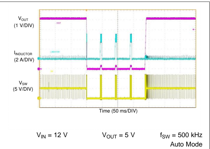
Figure 72. LM76003 Short-Circuit Behavior With Hiccup
