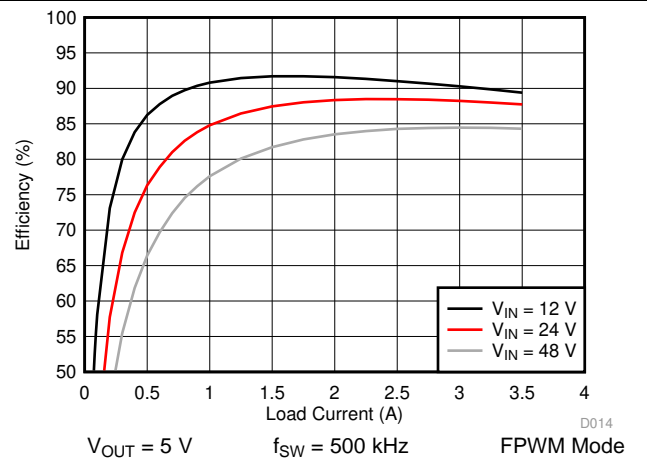
Figure 26. LM76003 Efficiency
