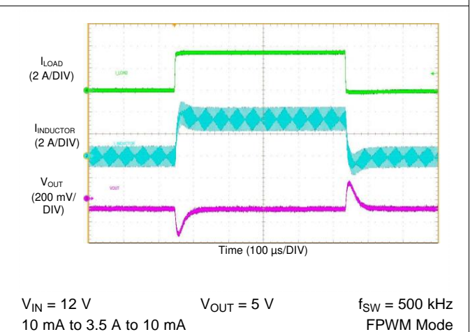
Figure 76. LM76003 Load Transient
