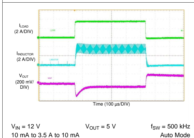
Figure 75. LM76003 Load Transient
