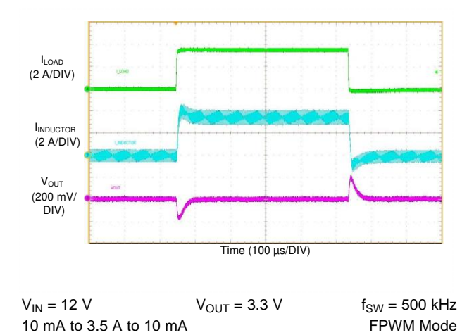
Figure 74. LM76003 Load Transient
