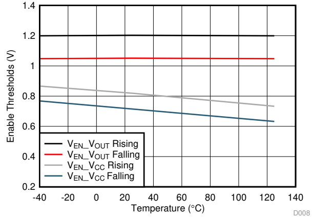
Figure 8. Enable Threshold
