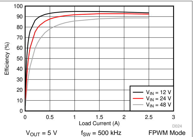
Figure 36. LM76002 Efficiency
