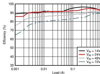
Typical Efficiency, V_{OUT} = 12\text{V}
