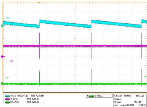
Figure 7-14. No-Load Switching
