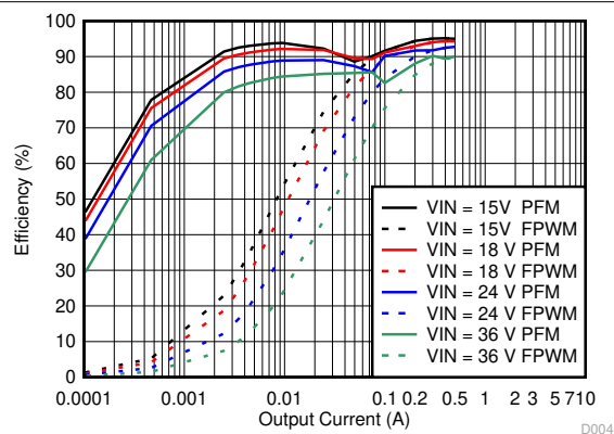
Figure 9-18. Efficiency
