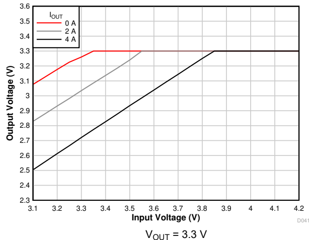
Figure 7-7. Voltage Dropout
