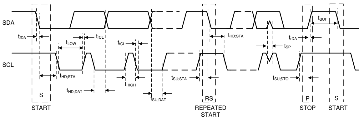
Figure 7-18. I²C-Compatible Timing
