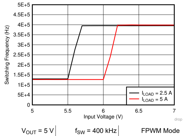
Figure 8-7. LM76005-Q1 Frequency Dropout
