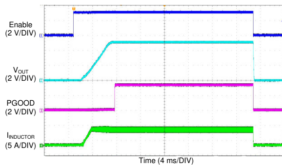
Figure 8-18. LM76005-Q1 Start-up Waveform
