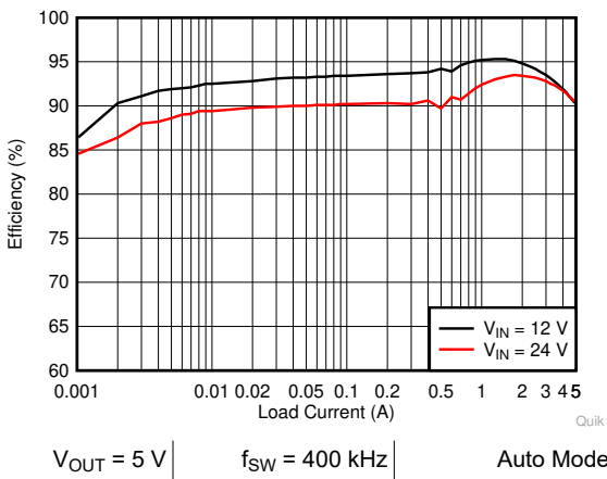
Figure 8-4. LM76005-Q1 Efficiency
