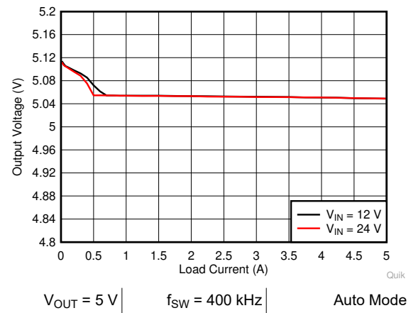
Figure 8-5. LM76005-Q1 Load and Line Regulation
