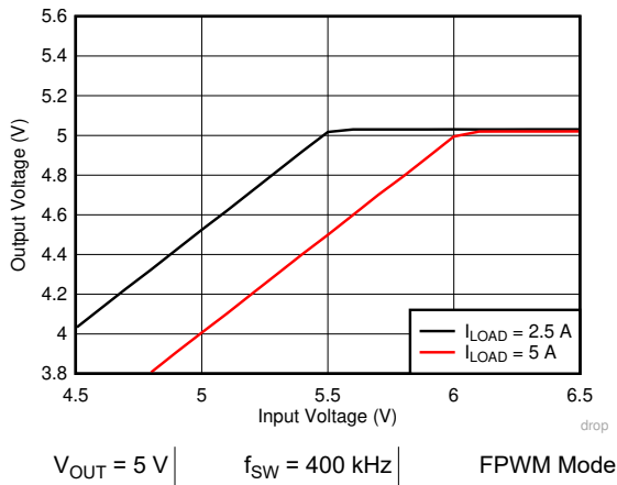
Figure 8-6. LM76005-Q1 Voltage Dropout
