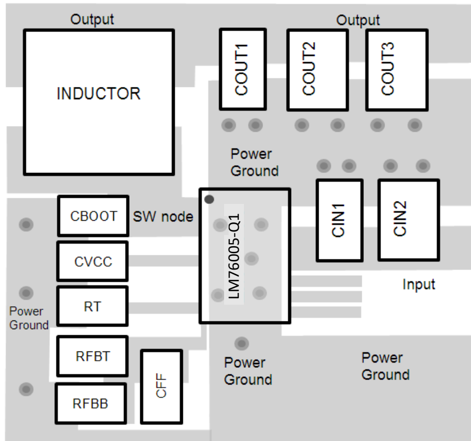
Figure 10-3. LM76005-Q1 Layout
