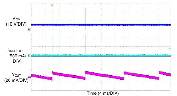
Figure 8-7. LM76005-Q1 Frequency Dropout
