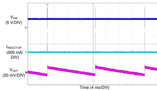
Figure 8-6. LM76005-Q1 Voltage Dropout
