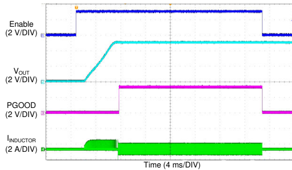
Figure 8-16. LM76005-Q1 Start-up Waveform
