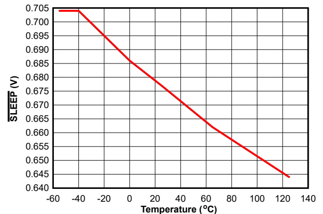
Figure 7-6. \overline{SLEEP} Logic High Threshold Voltage vs. Temperature
