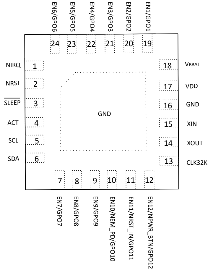
Figure 6-1. RGE Package 24-Pin VQFN TPS38700-Q1 Top View
