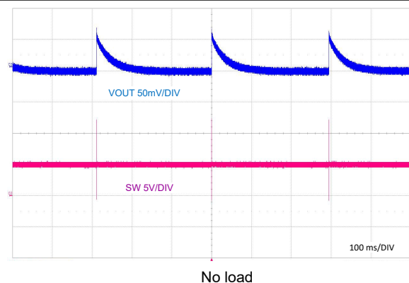
Figure 9-32. PFM Switching
