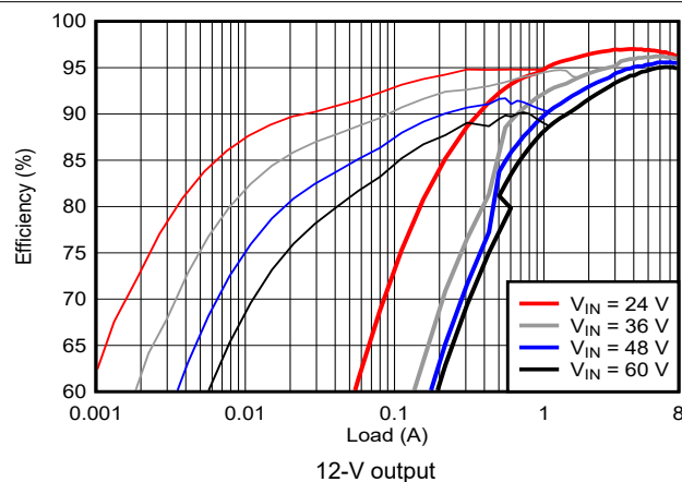
Figure 9-19. Efficiency vs. I_{OUT} , Log Scale
