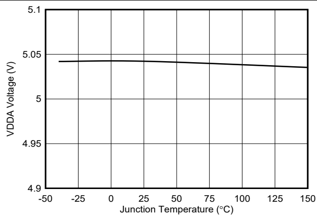
Figure 7-14. VDDA Regulation Voltage vs Temperature
