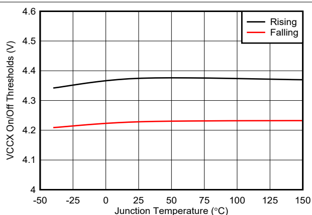
Figure 7-16. VCCX On, Off Thresholds vs Temperature
