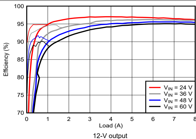
Figure 9-18. Efficiency vs. I_{OUT}
