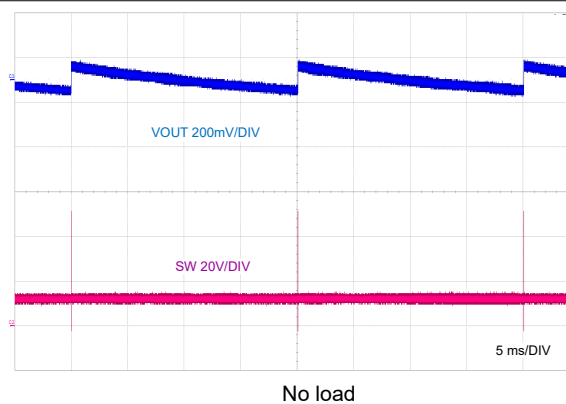
Figure 9-21. PFM Switching
