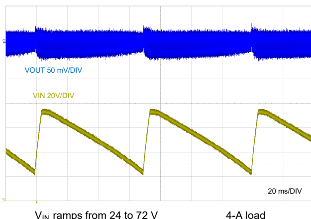
Figure 9-23. Line Transient Response to V_{IN} = 72\text{ V}
