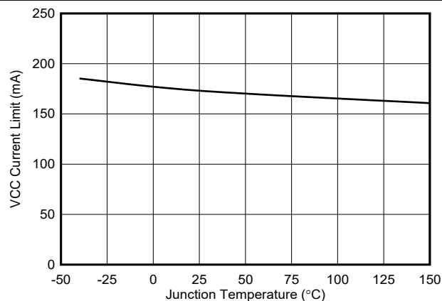
Figure 7-13. VCC Current Limit vs Temperature
