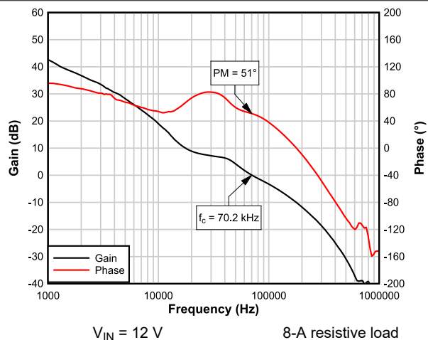
V_{IN} = 12 V 8-A resistive load Figure 9-15. Bode Plot, 5-V Output
