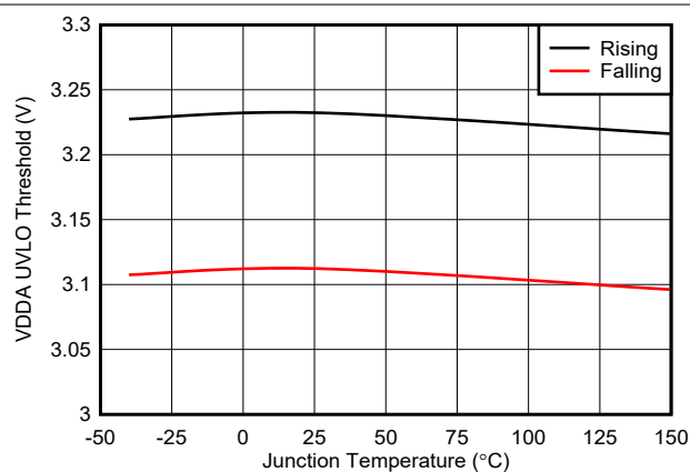
Figure 7-15. VDDA UVLO Thresholds vs Temperature
