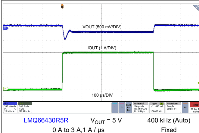
Figure 9-8. Load Transient
