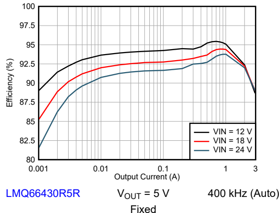
Figure 9-4. Efficiency
