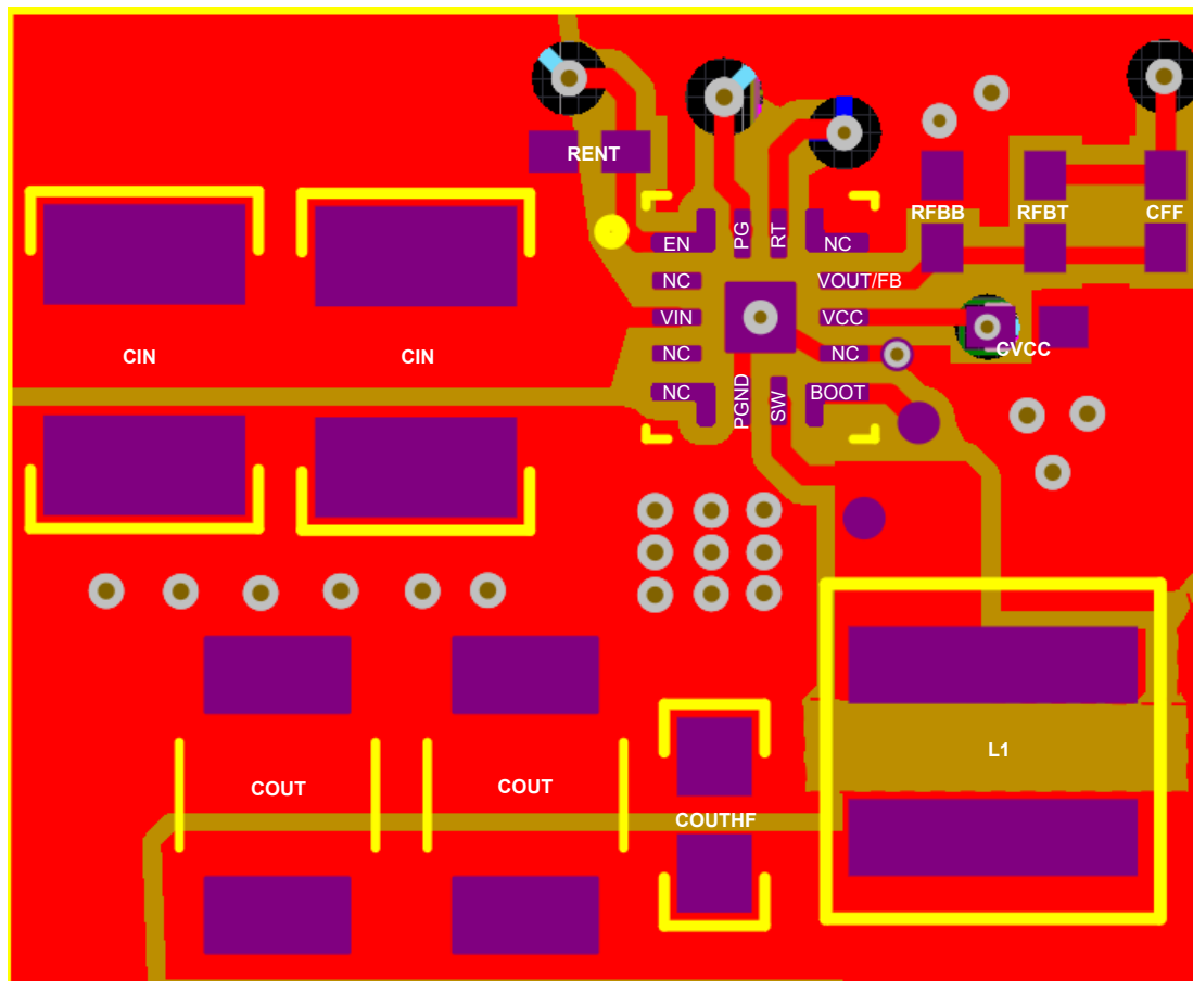
Figure 9-13. Example Layout
