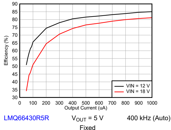
Figure 9-5. Efficiency
