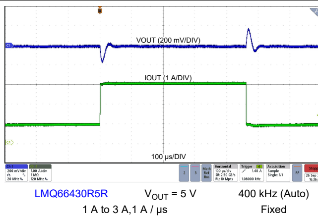
Figure 9-9. Load Transient
