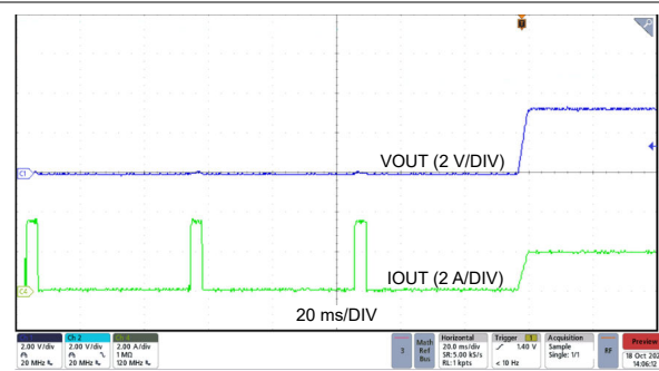
Figure 8-12. Hiccup Exit
