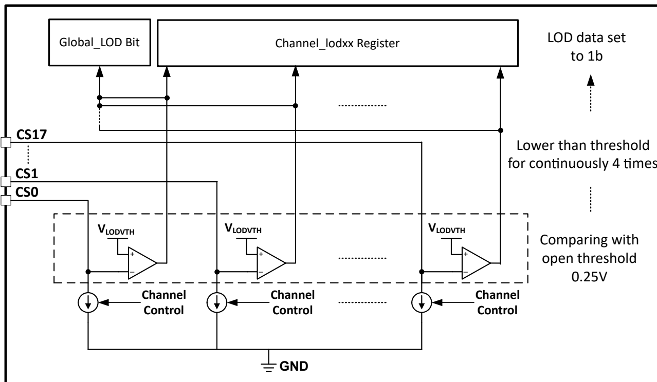
Figure 7-11. LOD Circuits
