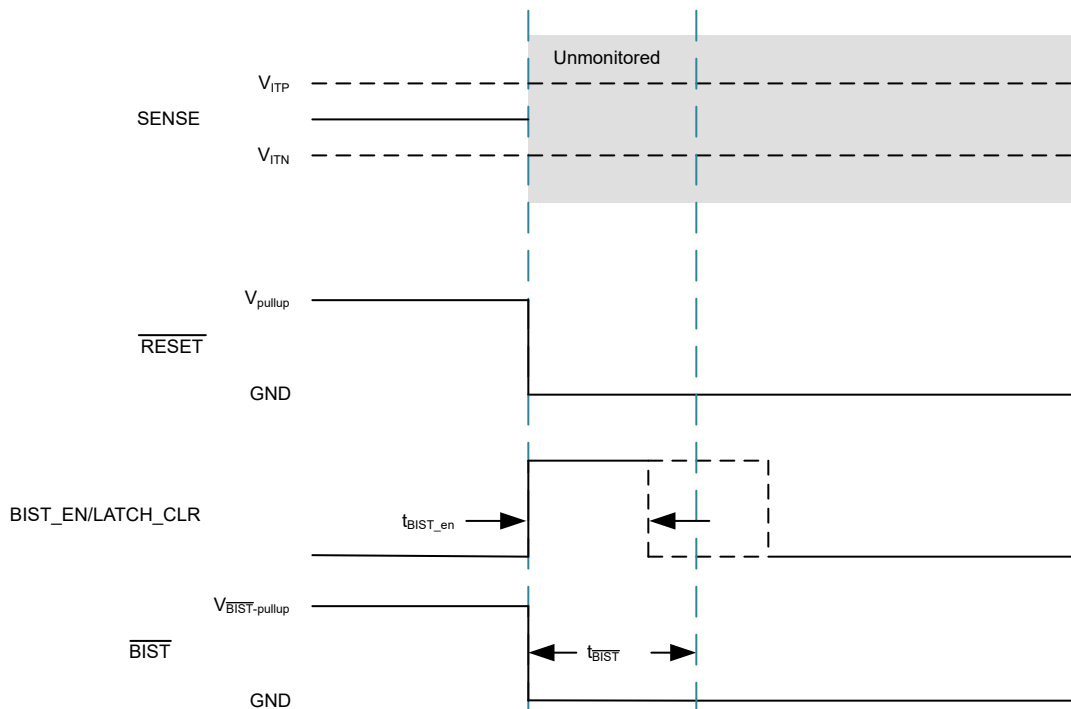
Figure 10-13. \overline{BIST} Fail With \overline{RESET} Assertion
