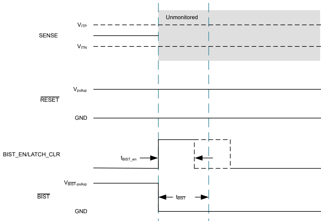
Figure 10-14. \overline{BIST} Fail With No \overline{RESET} Assertion
