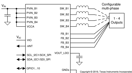
Simplified Schematic
