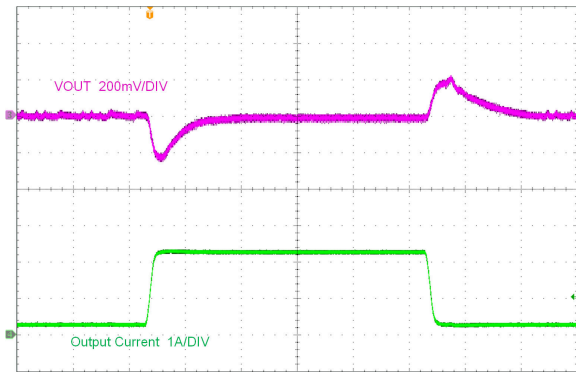
LMR38025(PFM) V_{OUT} = 5V 400kHz, 100 \mu s/DIV (AC Coupled) 250mA to 2.25A at 200mA/ \mu s
