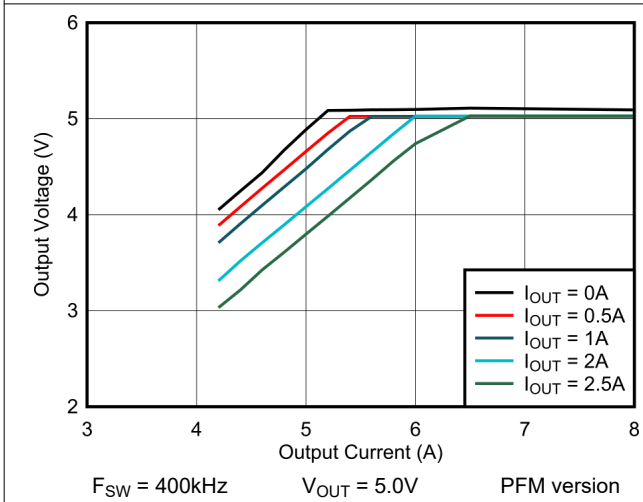
Figure 6-3. 5V Dropout
