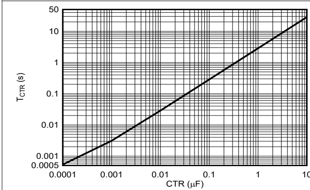
Figure 6-5. T_{\text{CTR}} vs CTR
