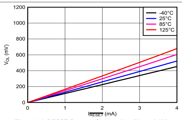
Figure 6-8. RESET Current (Sink) vs V_{\text{OL}} ( V_{\text{DD}} = 3.3\text{V} )
