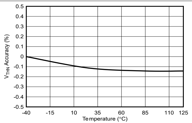
Figure 6-4. V_{\text{THN}} Accuracy vs Temperature
