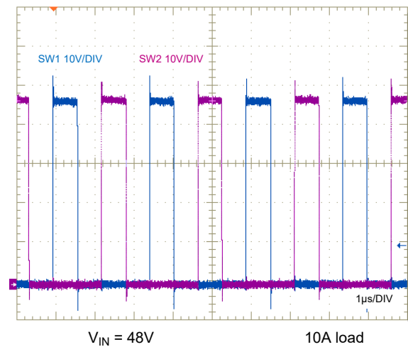
Figure 8-26. Switch-node Voltages
