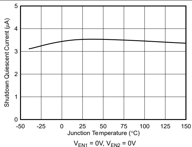
Figure 6-7. Shutdown Quiescent Current vs Temperature
