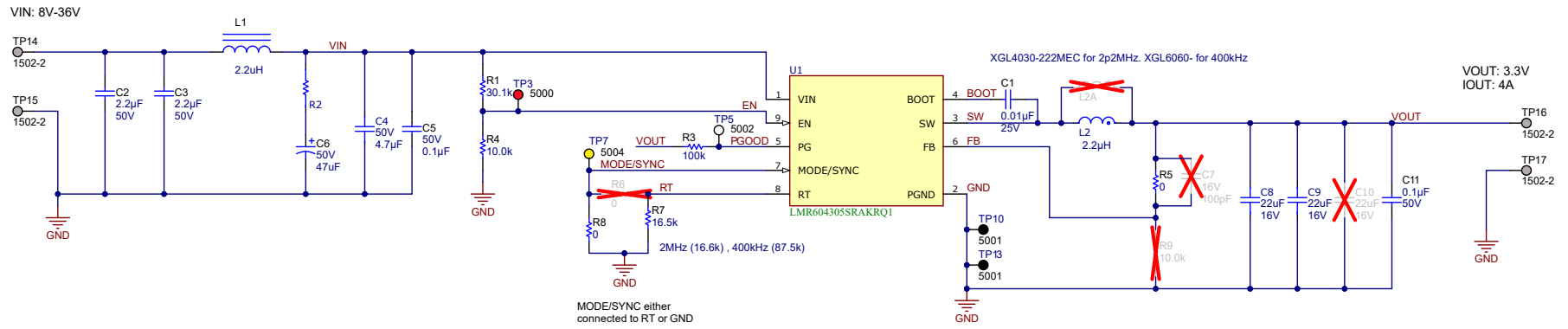
Figure 4-1. LMR60440QEVM Schematic
