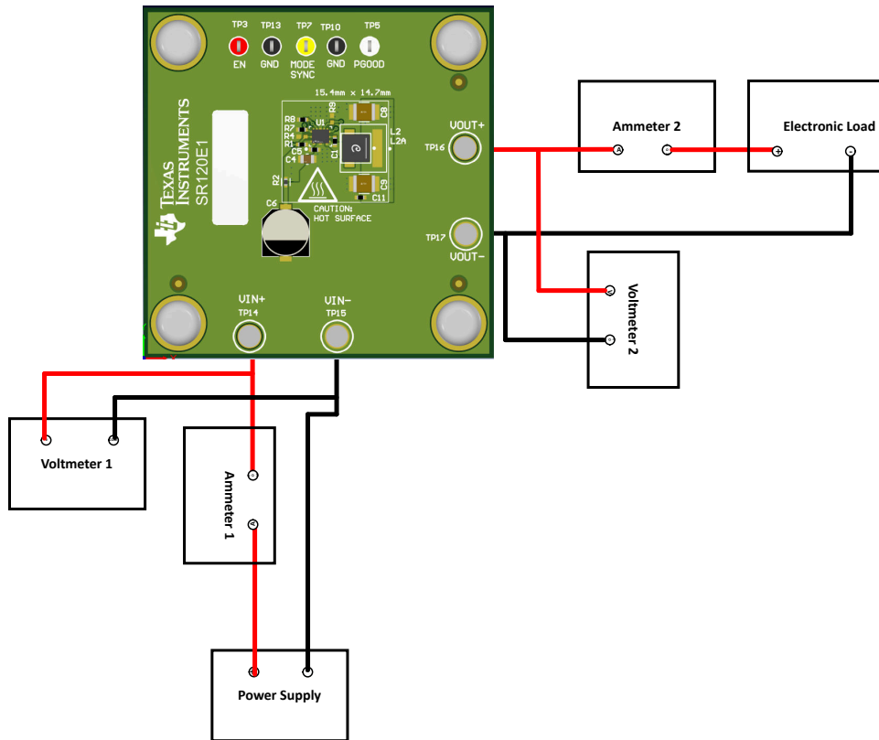
Figure 2-1. EVM Board Connections
