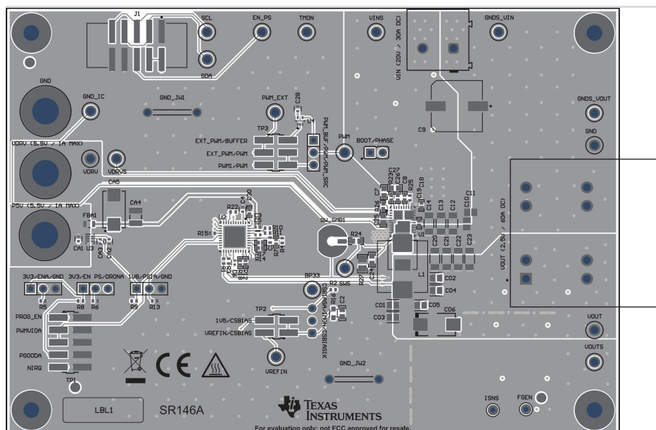
Figure 4-3. SR146A CSD967201-Q1EVM Top Composite View (Top View)
