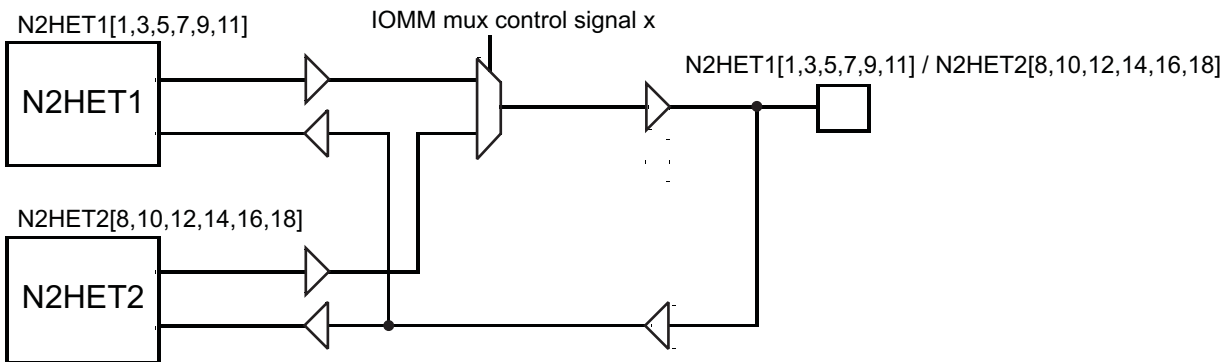
Figure 7-18. N2HET Monitoring
