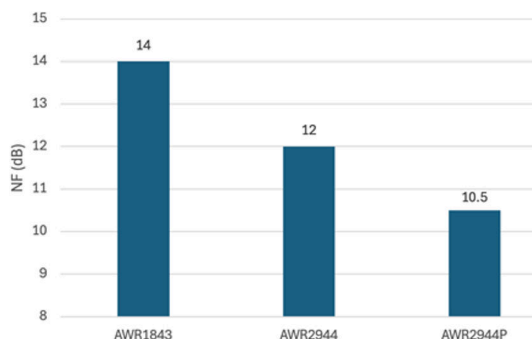
Figure 3-4. Noise figure enhancements on AWR2944P
