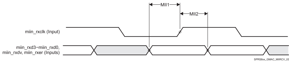
Figure 5-70. GMAC Receive Interface Timing MIIIn operation
