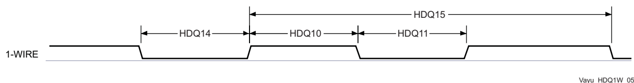
Figure 5-46. 1-Wire—Break (Reset)
