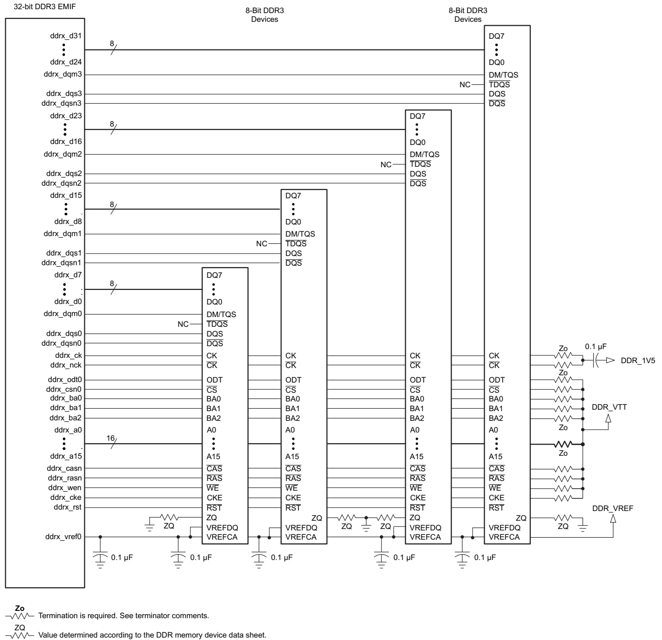
Figure 7-3. 32-Bit, One-Bank DDR3 Interface Schematic Using Four 8-Bit DDR3 Devices
