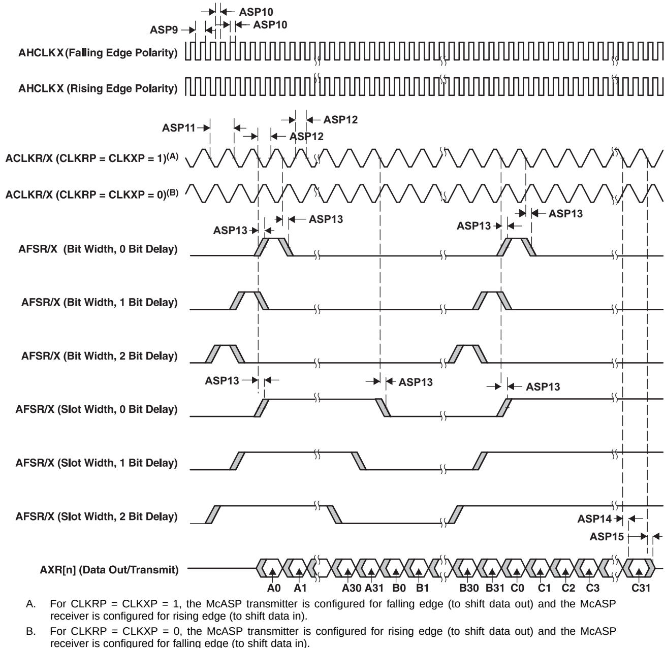
Figure 5-51. McASP Output Timing
