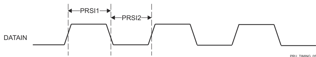
Figure 6-112. PRUSS PRU Shift In Timing
