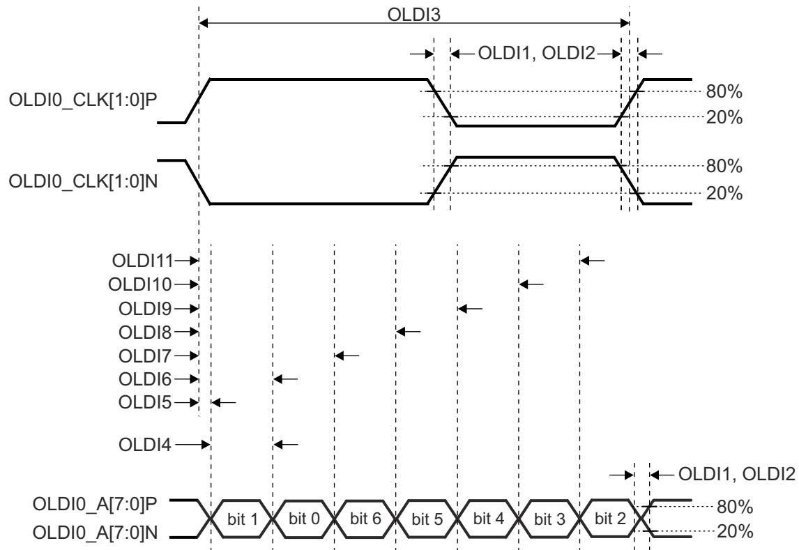
Figure 6-95. OLDI0 Switching Characteristics
