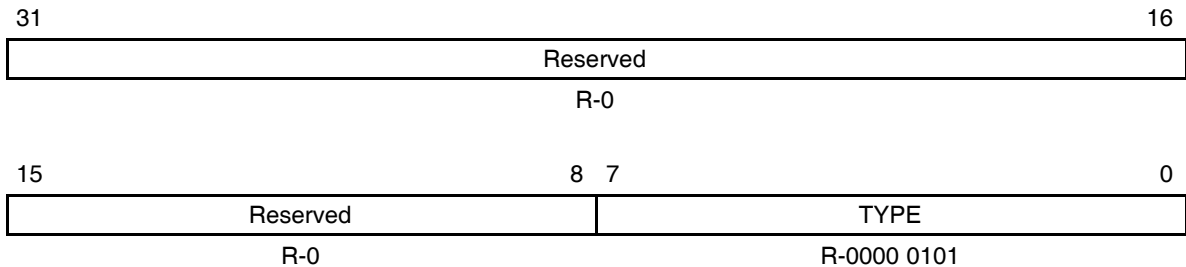
Figure B–153. I2C Peripheral Identification Register 2 (I2CPID2)
