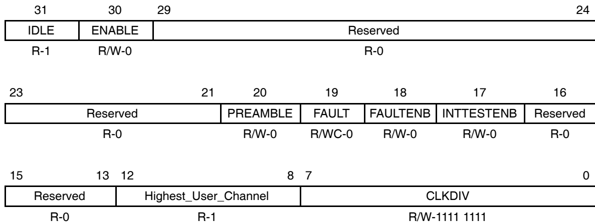
Figure B–219. MDIO Control Register (CONTROL)
