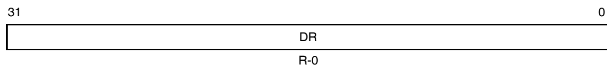
Figure B–206. Data Receive Register (DRR)
