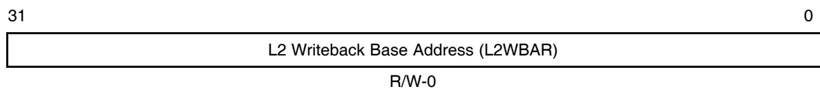
Figure B–3. L2 Writeback Base Address Register (L2WBAR)
