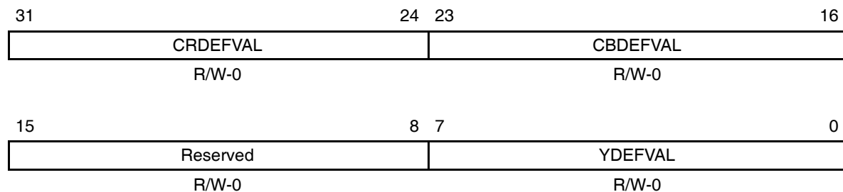
Figure B–342. Video Display Default Display Value Register (VDDEFVAL)
