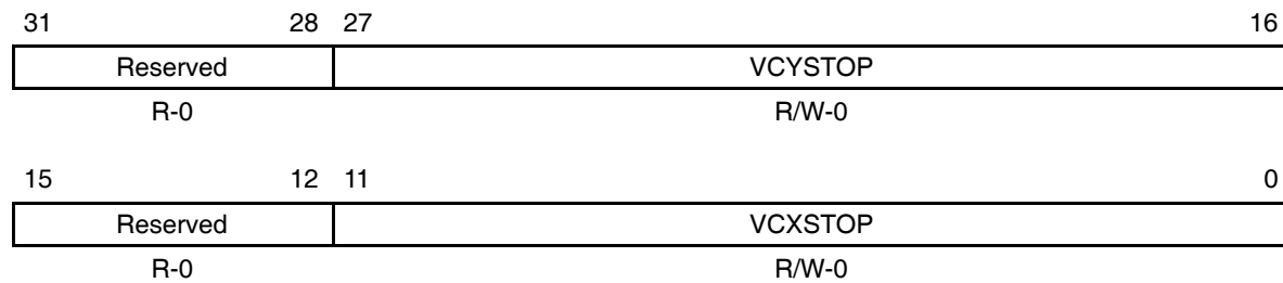
Figure B–302. Video Capture Channel x Field 1 Stop Register (VCASTOP1, VCBSTOP1)
