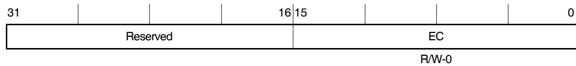
Figure B–56. EDMA Event Clear Register (ECR)
