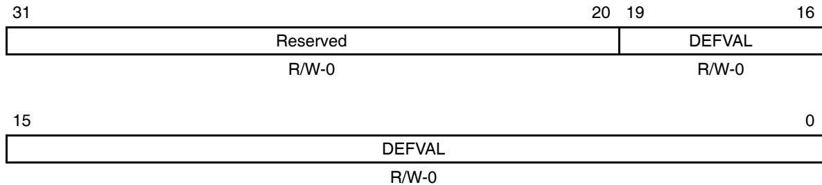
Figure B–343. Video Display Default Display Value Register (VDDEFVAL)—Raw Data Mode
