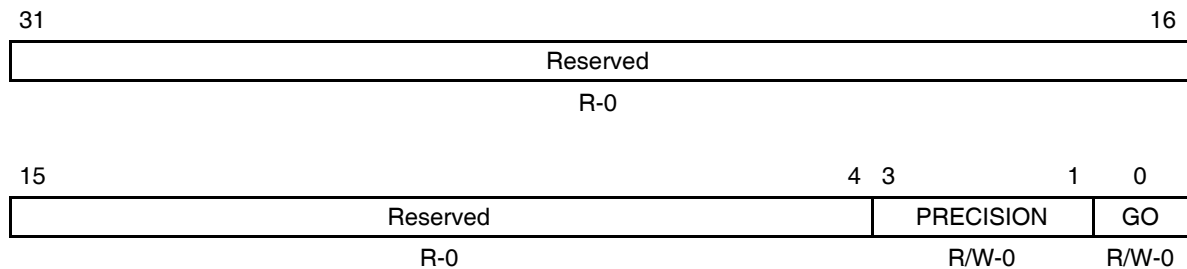
Figure B–292. VIC Control Register (VICCTL)
