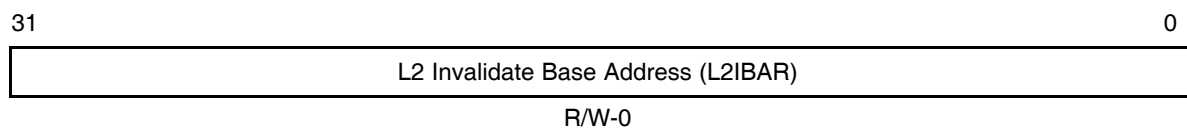
Figure B–7. L2 Invalidate Base Address Register (L2IBAR)
