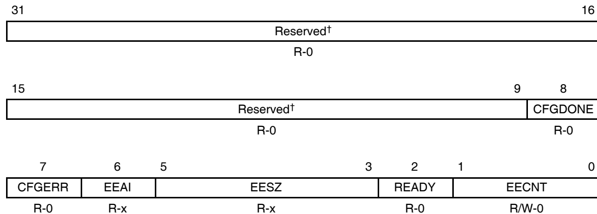
Figure B–244. EEPROM Control Register (EECTL)
