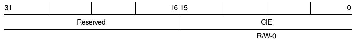
Figure B–45. EDMA Channel Interrupt Enable Register (CIER)
