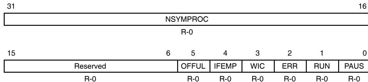
Figure B–289. VCP Status Register 0 (VCPSTAT0)
