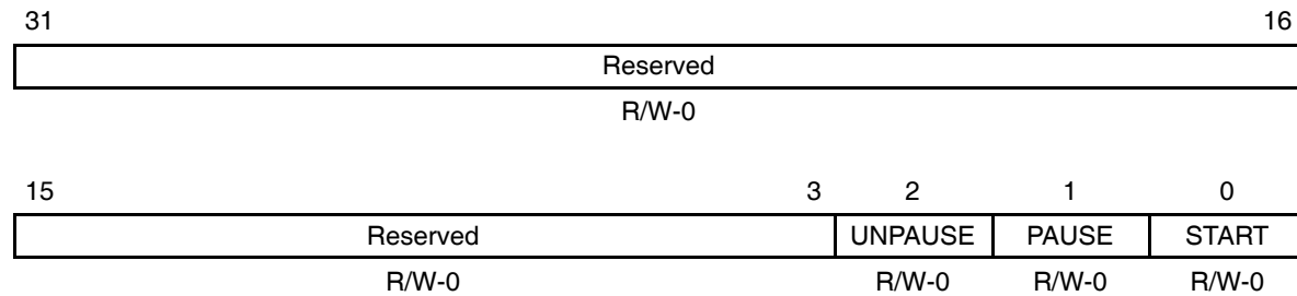
Figure B–266. TCP Execution Register (TCPEXE)
