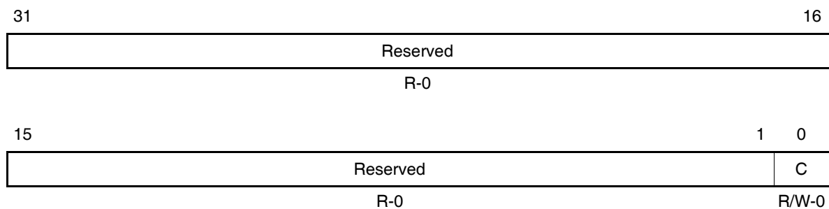
Figure B–17. L2 Writeback-Invalidate All Register (L2WBINV)
