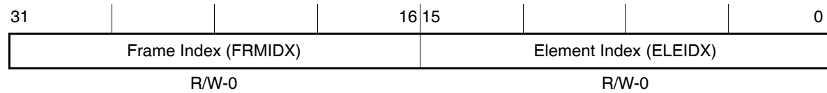
Figure B–28. DMA Global Index Register (GBLIDX)
