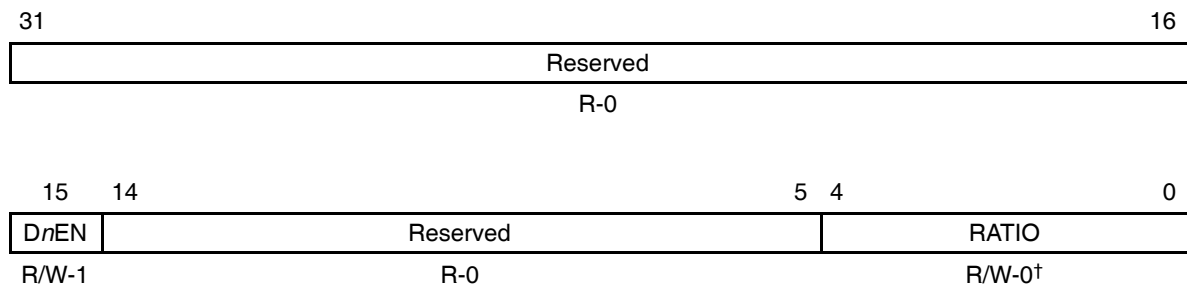
Figure B–250. PLL Controller Divider Register (PLLDIV)
