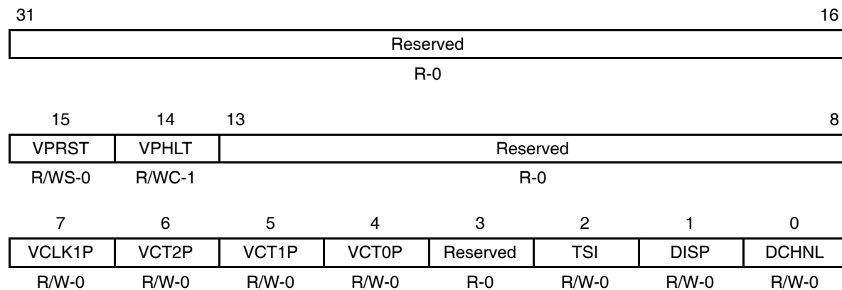
Figure B–295. Video Port Control Register (VPCTL)
