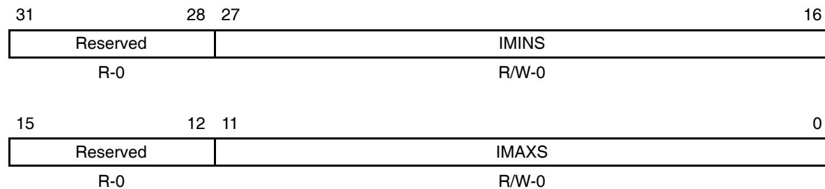
Figure B–283. VCP Input Configuration Register 4 (VCPIC4)
