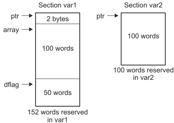
Figure 5-7. The .usect Directive
