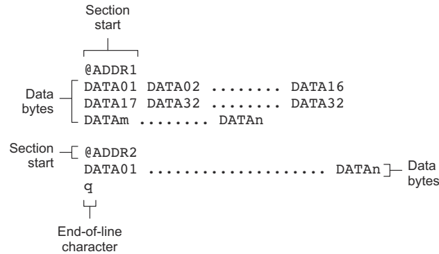
Figure 12-14. TI-TXT Object Format
