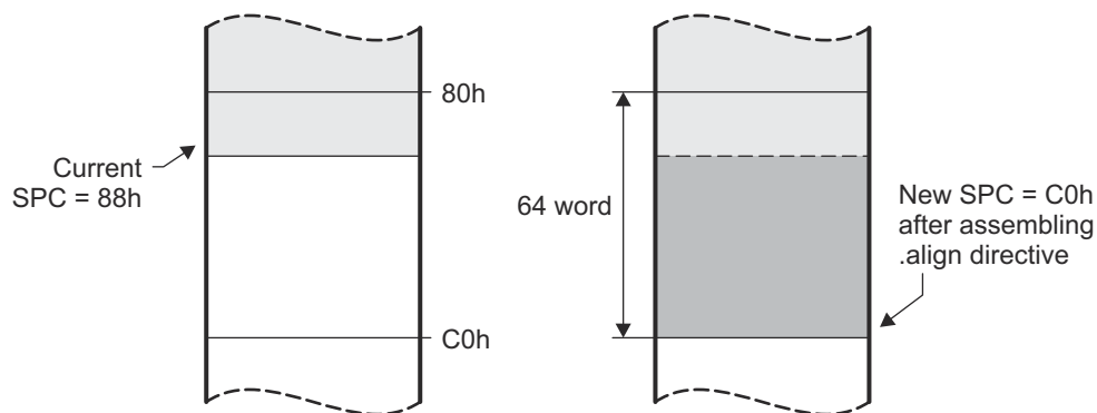
Figure 5-3. The .align Directive
