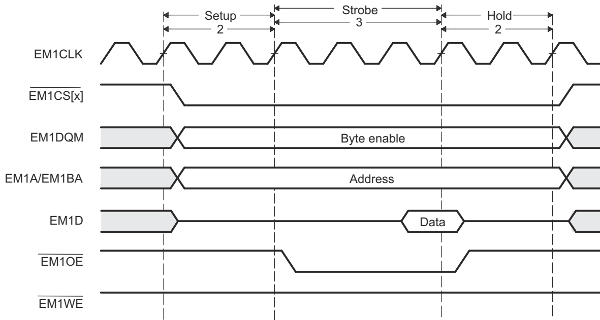
Figure 13-11. Timing Waveform of an Asynchronous Read Cycle in Normal Mode
