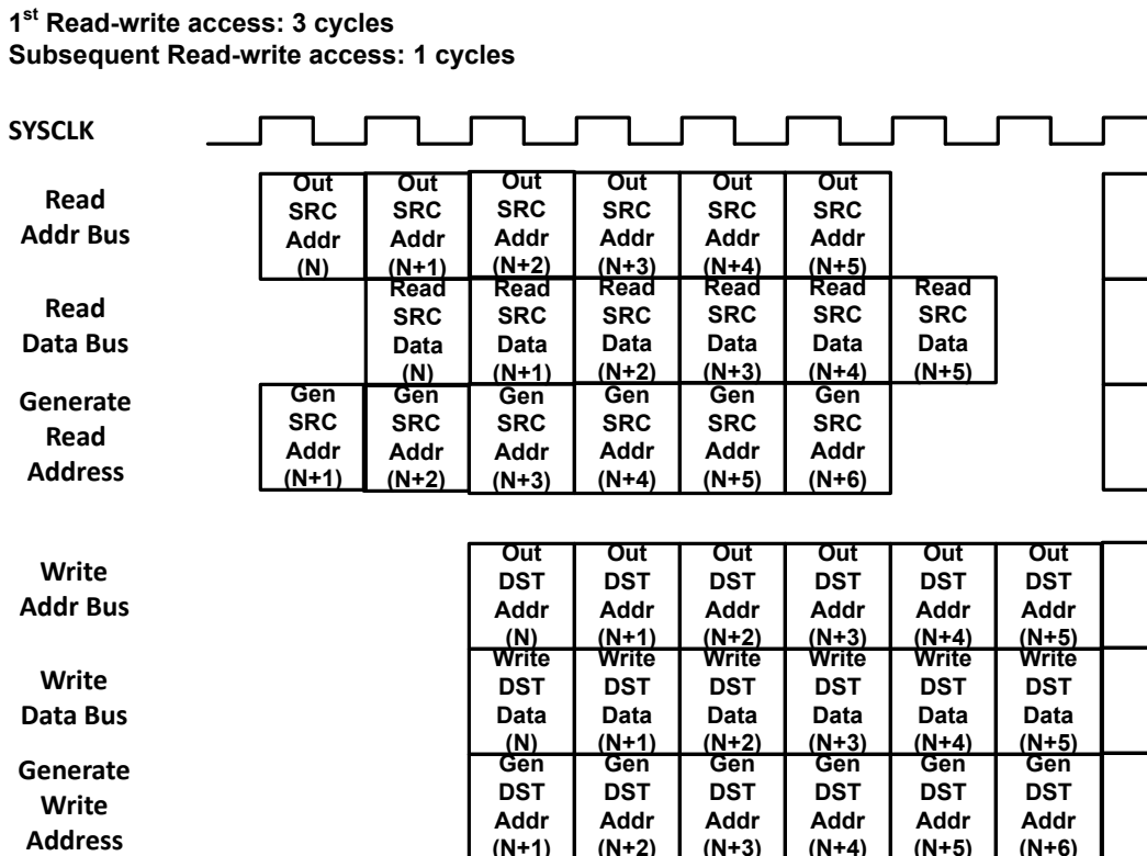
Figure 12-3. 3-stage Pipeline: With 0 Cycle Read Stall and 0 Cycle Write Stall
