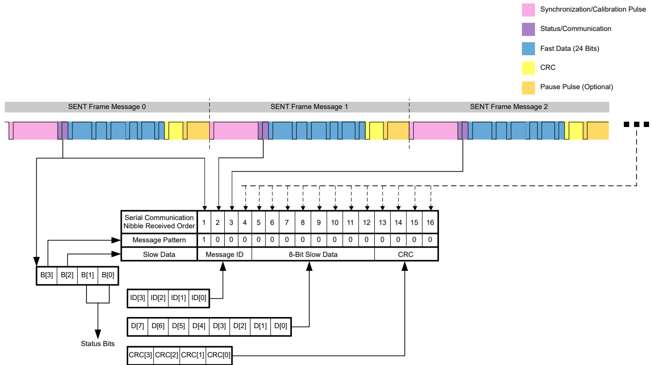
Figure 38-5. Short Serial Message
