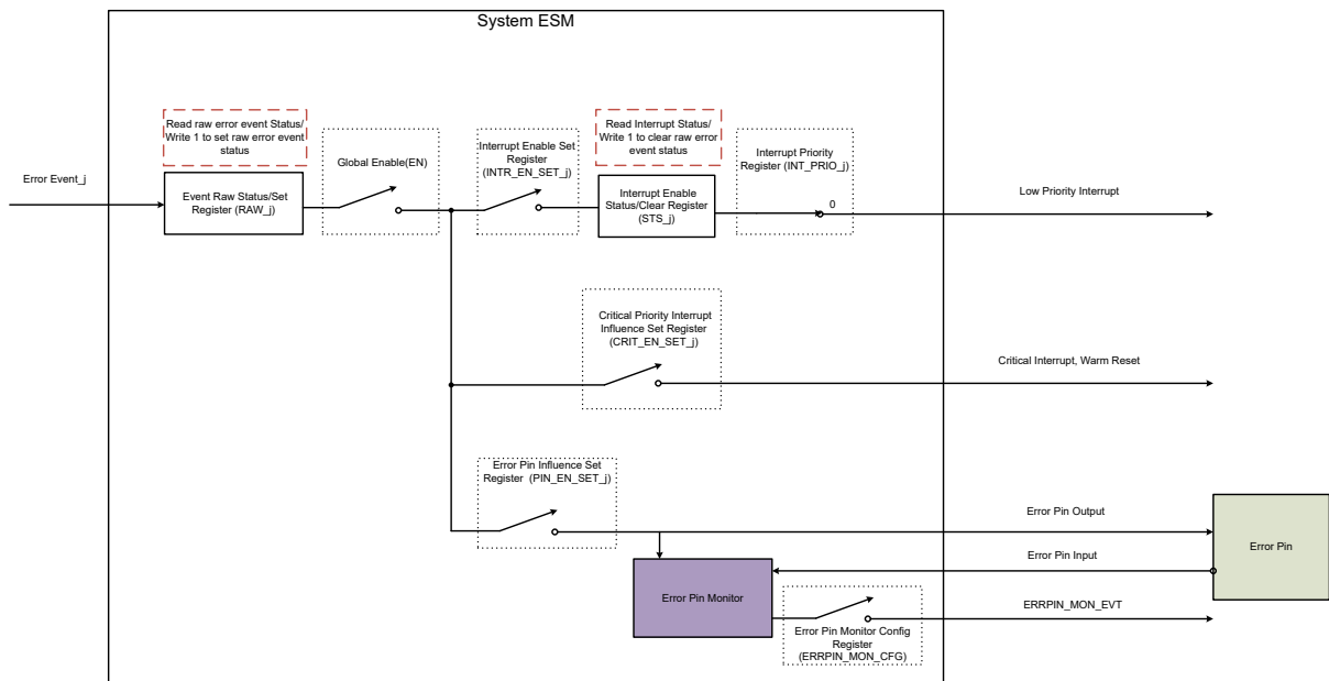
Figure 7-15. ESM CPU Register Configuration View
