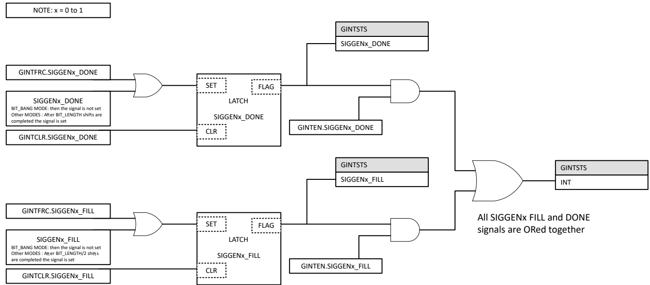
Figure 20-7. EPG Interrupt
