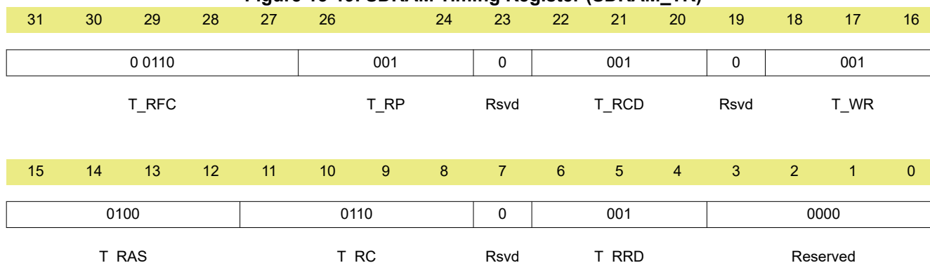
Figure 13-19. SDRAM Timing Register (SDRAM_TR)
