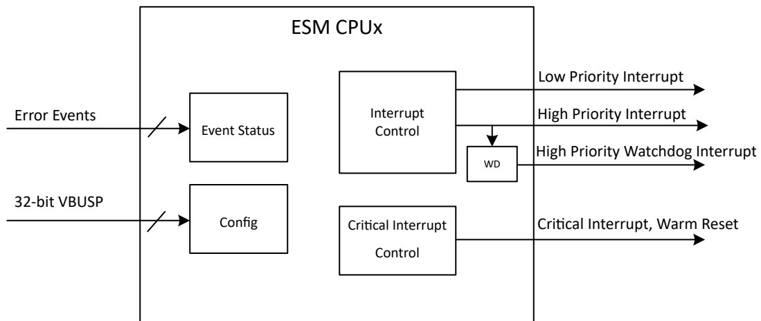
Figure 7-5. ESM CPU Block Diagram
