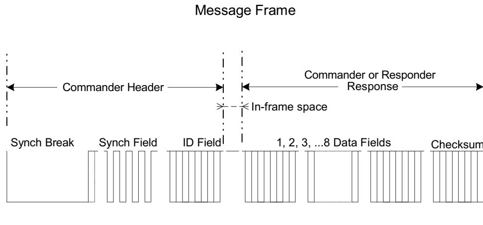
Figure 36-12. LIN Protocol Message Frame Format: Commander Header and Responder Peripheral Response
