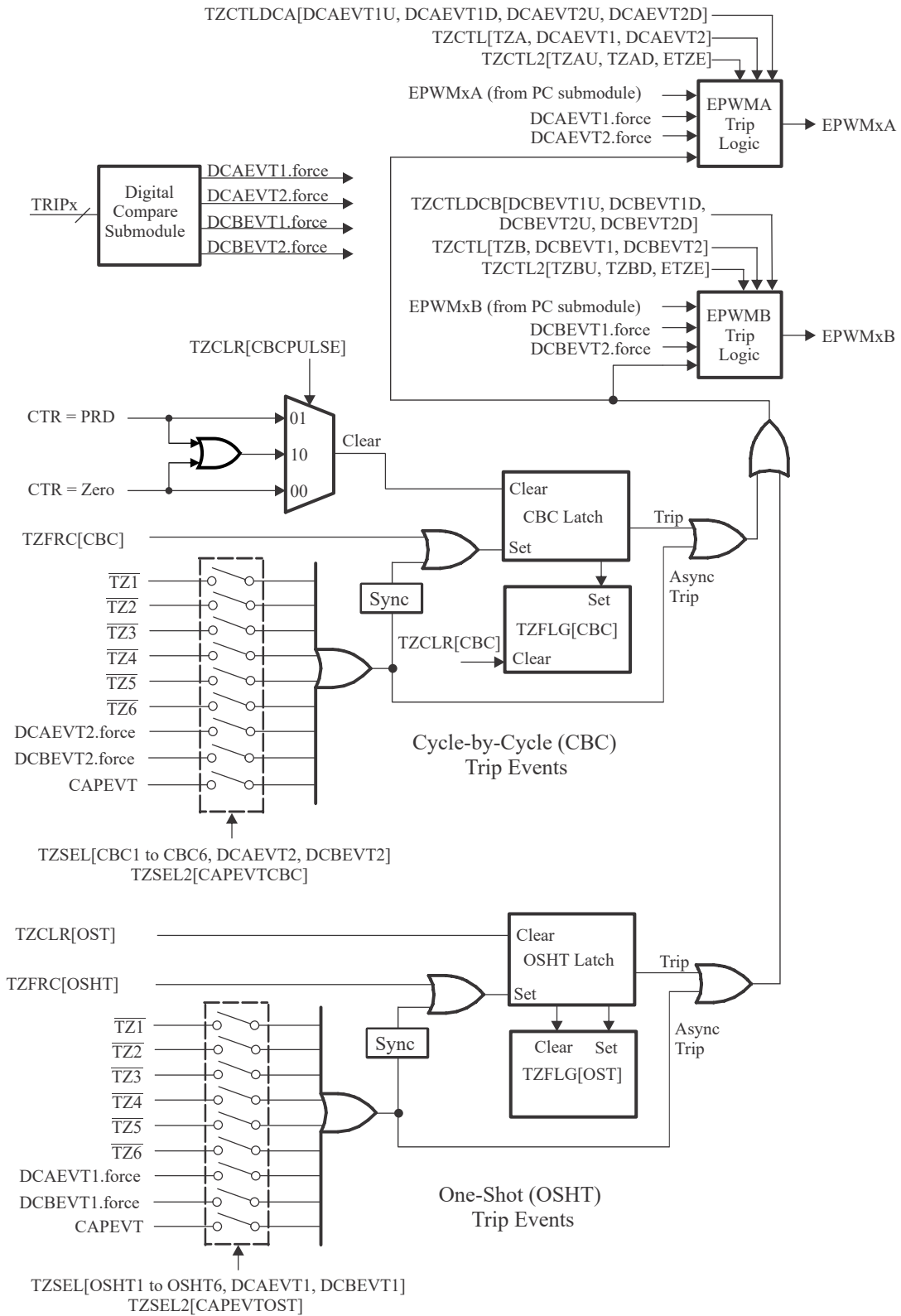
Figure 27-50. Trip-Zone Submodule Mode Control Logic
