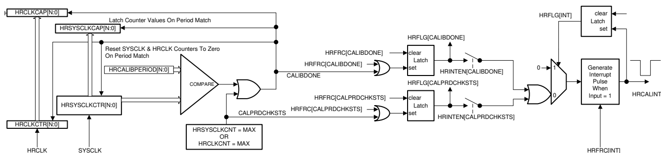
Figure 26-2. HRCAP Calibration
