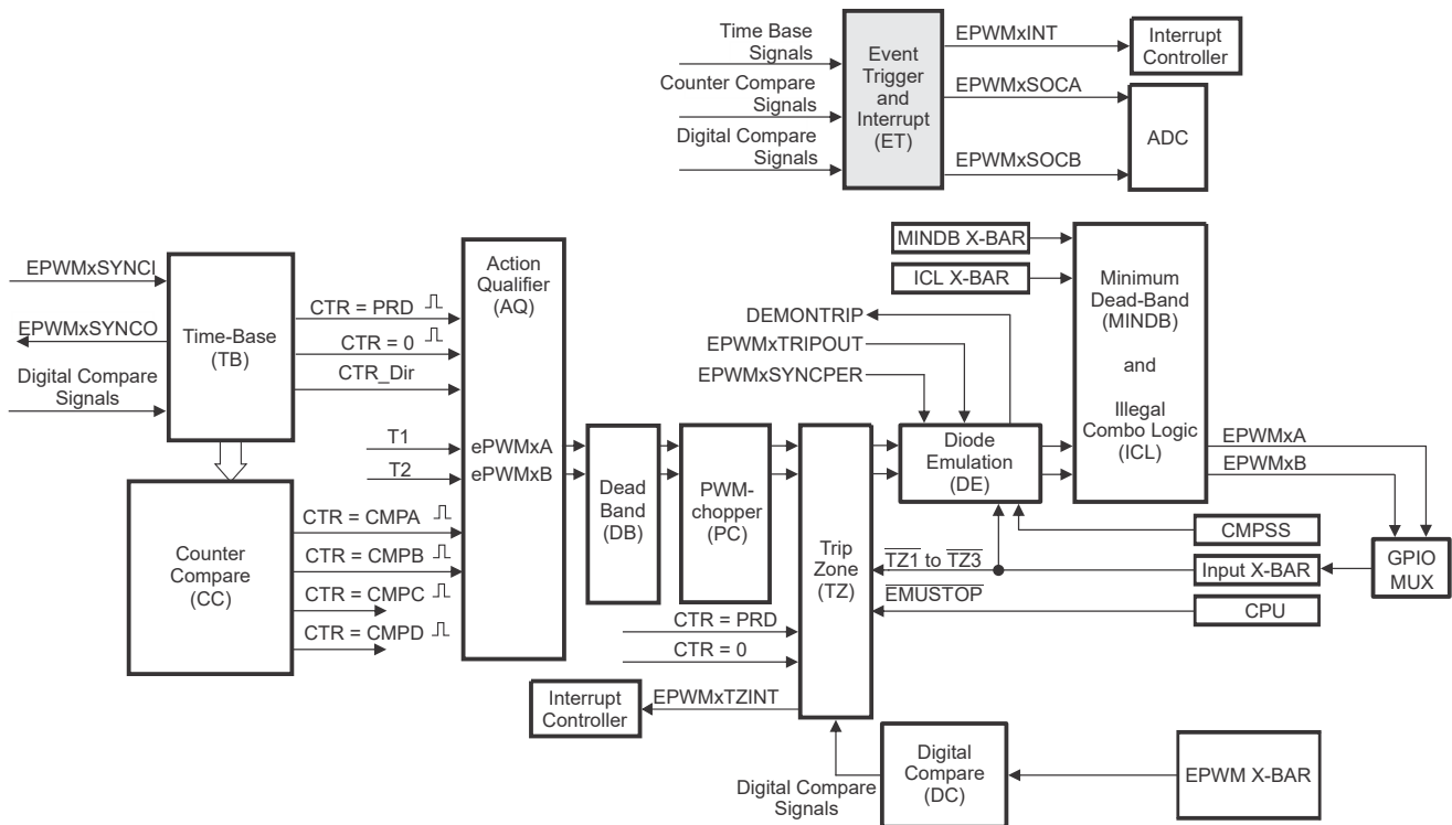
Figure 27-69. Event-Trigger Submodule
