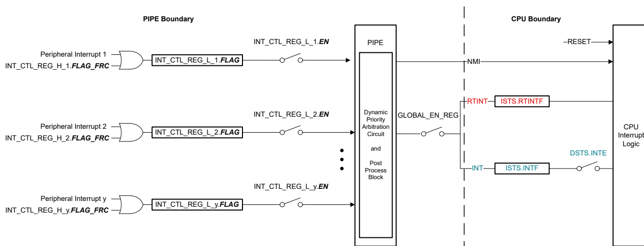
Figure 5-2. Interrupt Propagation
