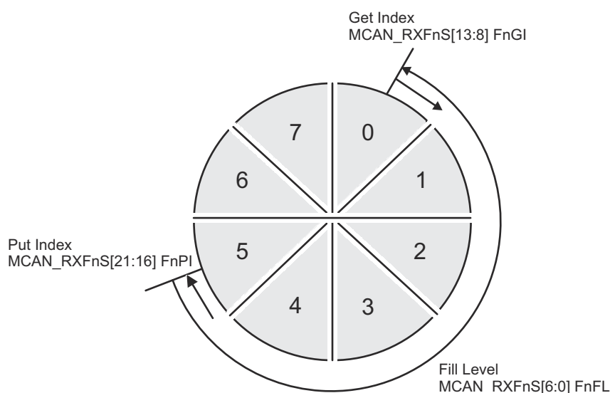
Figure 30-15. Rx FIFO Status
