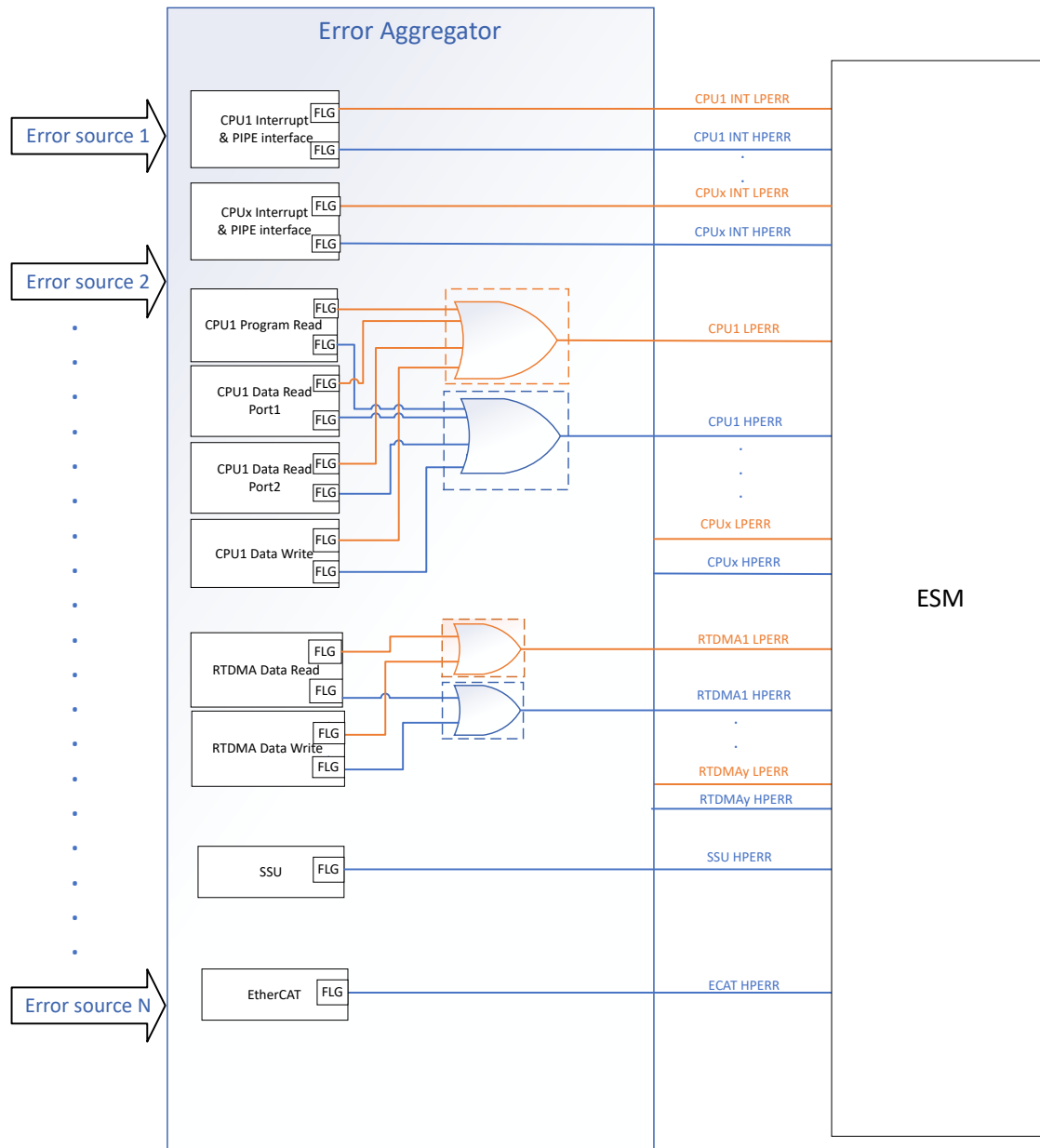
Figure 6-3. Error Aggregator Interface
