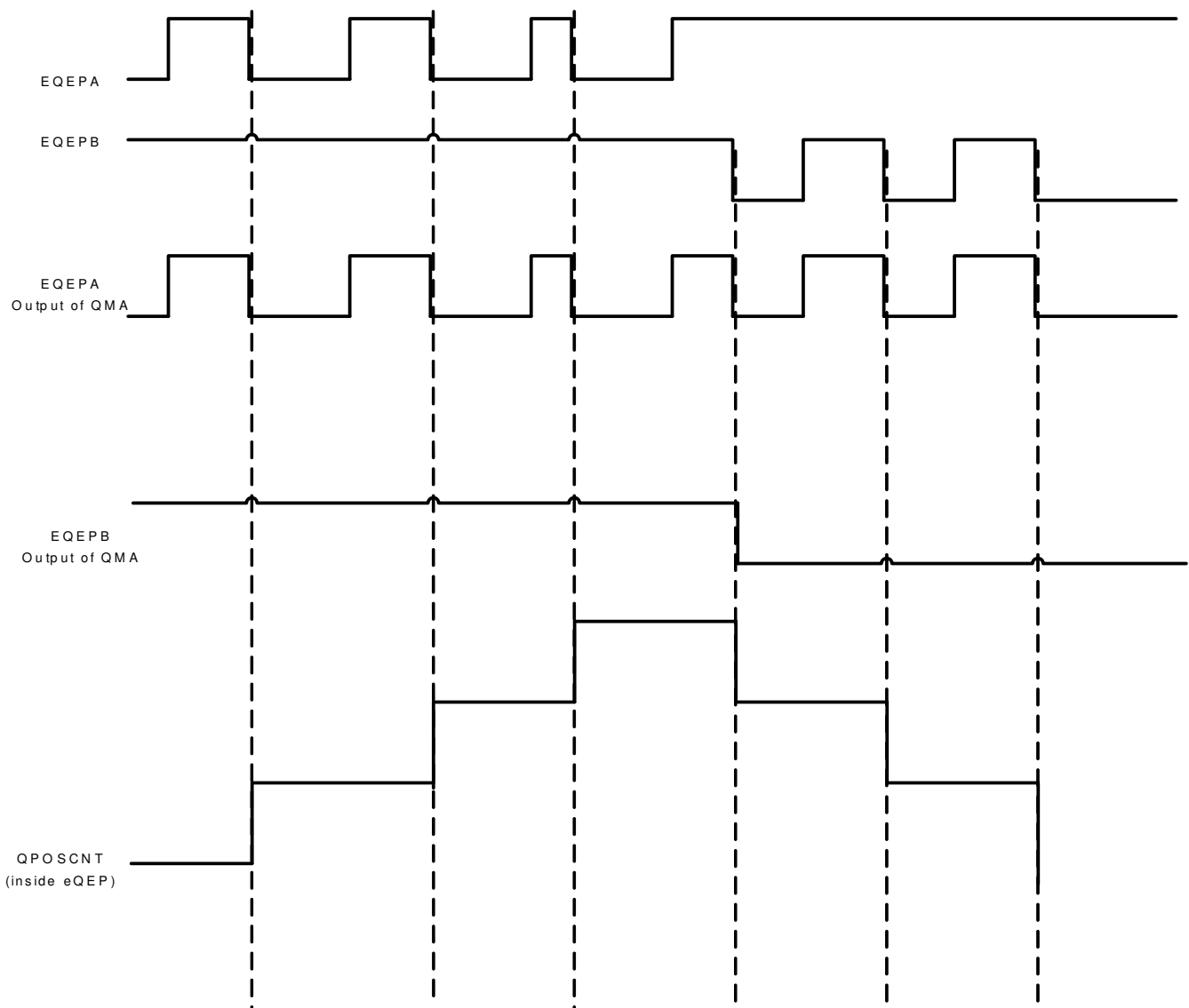
Figure 28-23. QMA Mode-1
