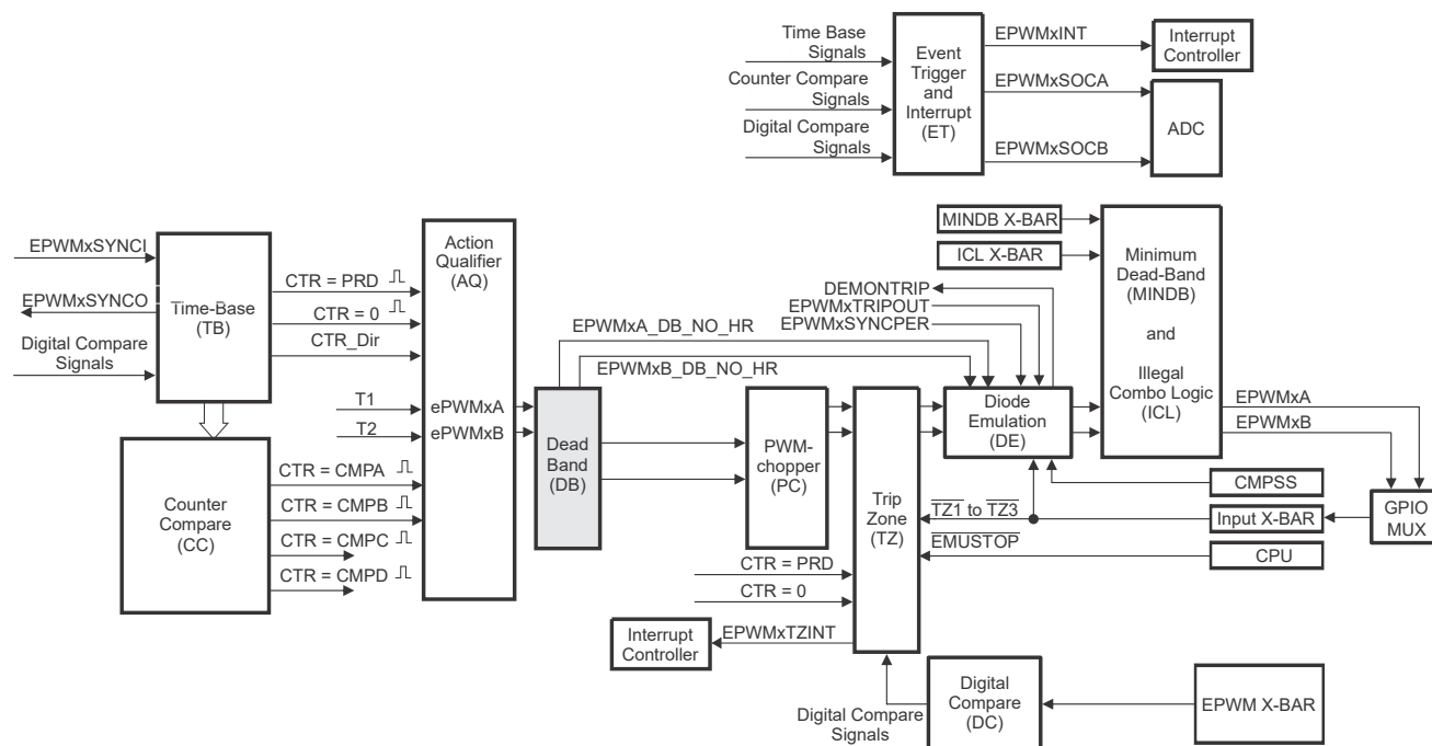
Figure 27-40. Dead_Band Submodule
