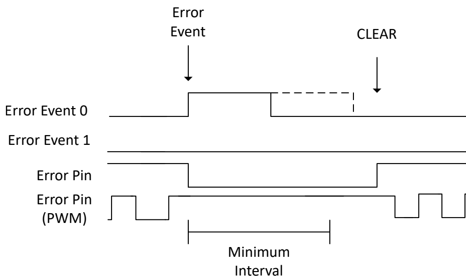
Figure 7-11. Error Pin Asserting with CLEAR after Minimum Interval
