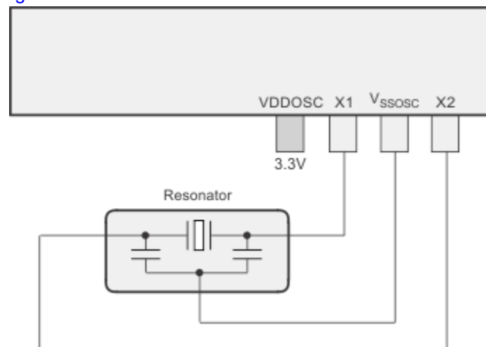
Figure 2-7. External Resonator
