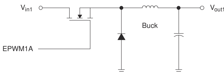
Figure 27-118. Simple Buck Controlled Converter Using a Single PWM
