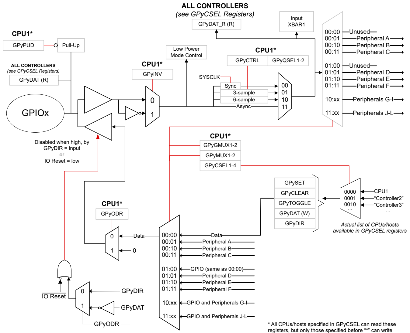
Figure 14-1. GPIO Logic for a Single Pin
