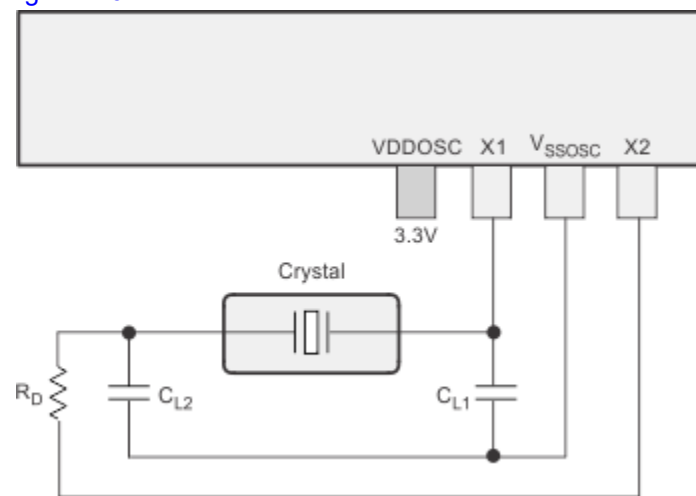
Figure 2-6. External Crystal
