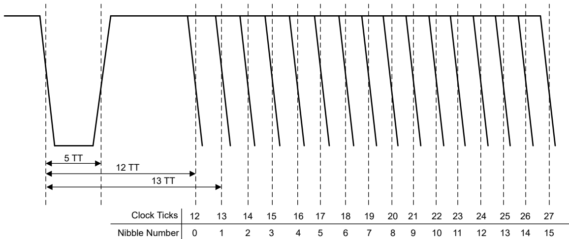
Figure 38-3. Nibble Pulse
