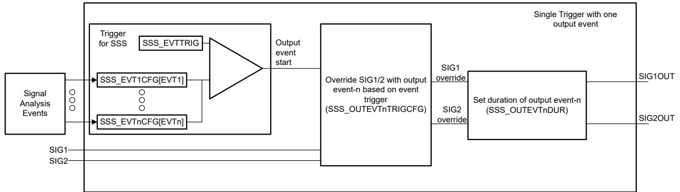
Figure 18-9. Single Trigger with Single Pattern Output Event
