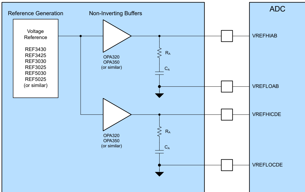
Figure 22-43. ADC Reference System
