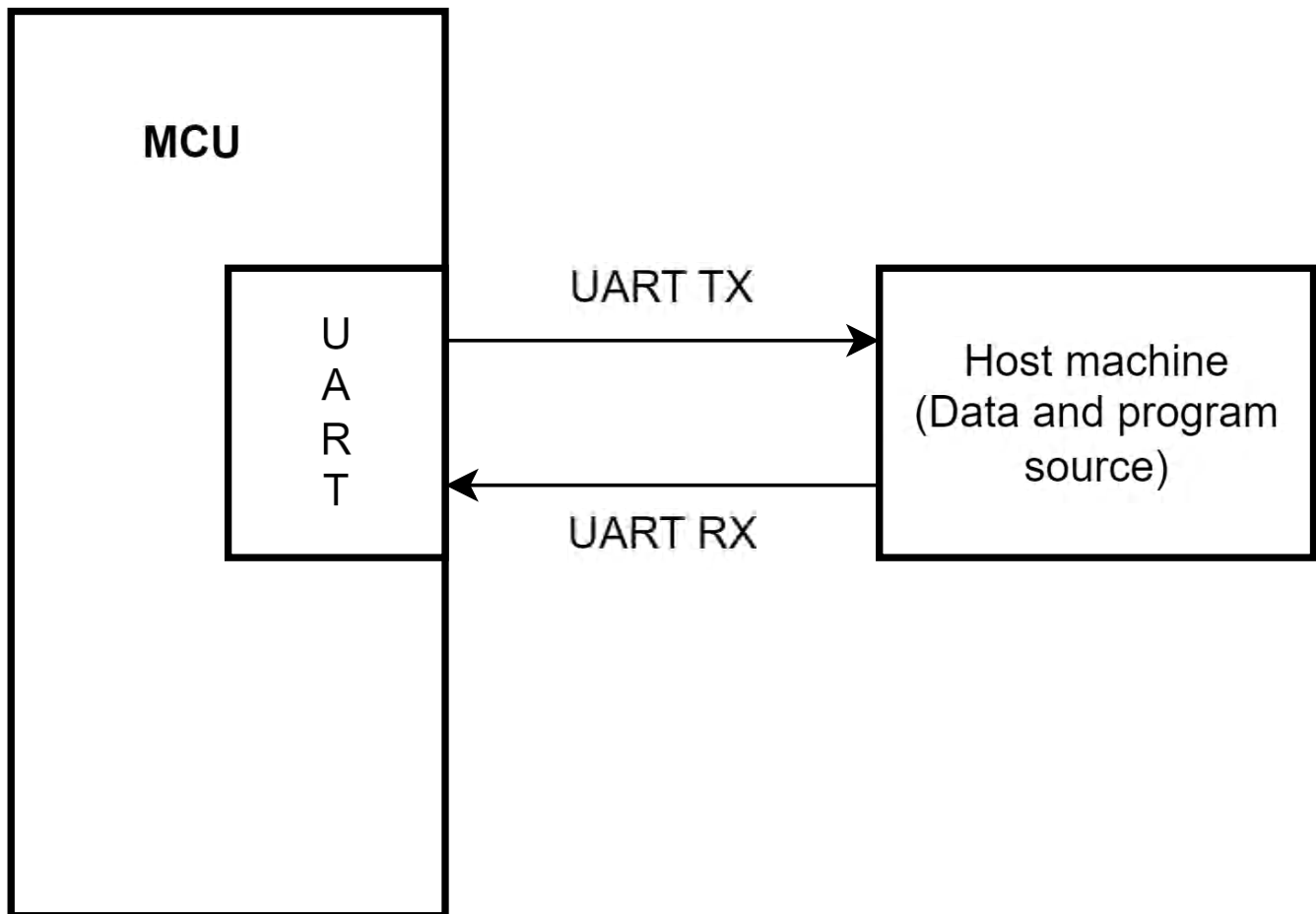
Figure 3-13. UART Boot Mode
