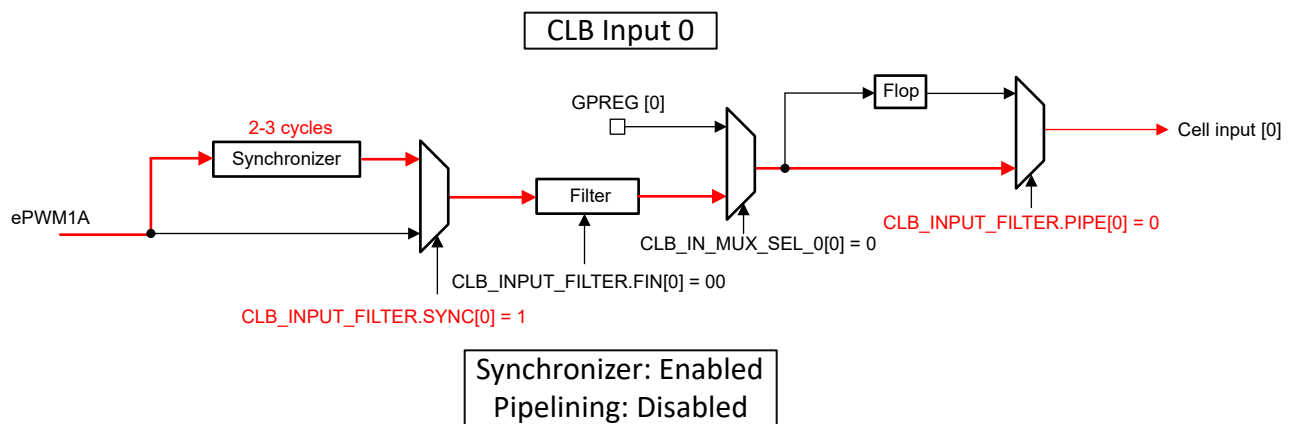
Figure 10-7. CLB Input Synchronization Example
