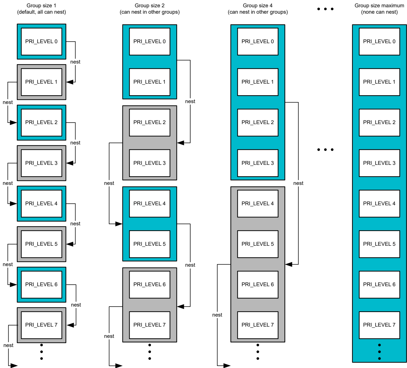
Figure 5-3. Interrupt Grouping
