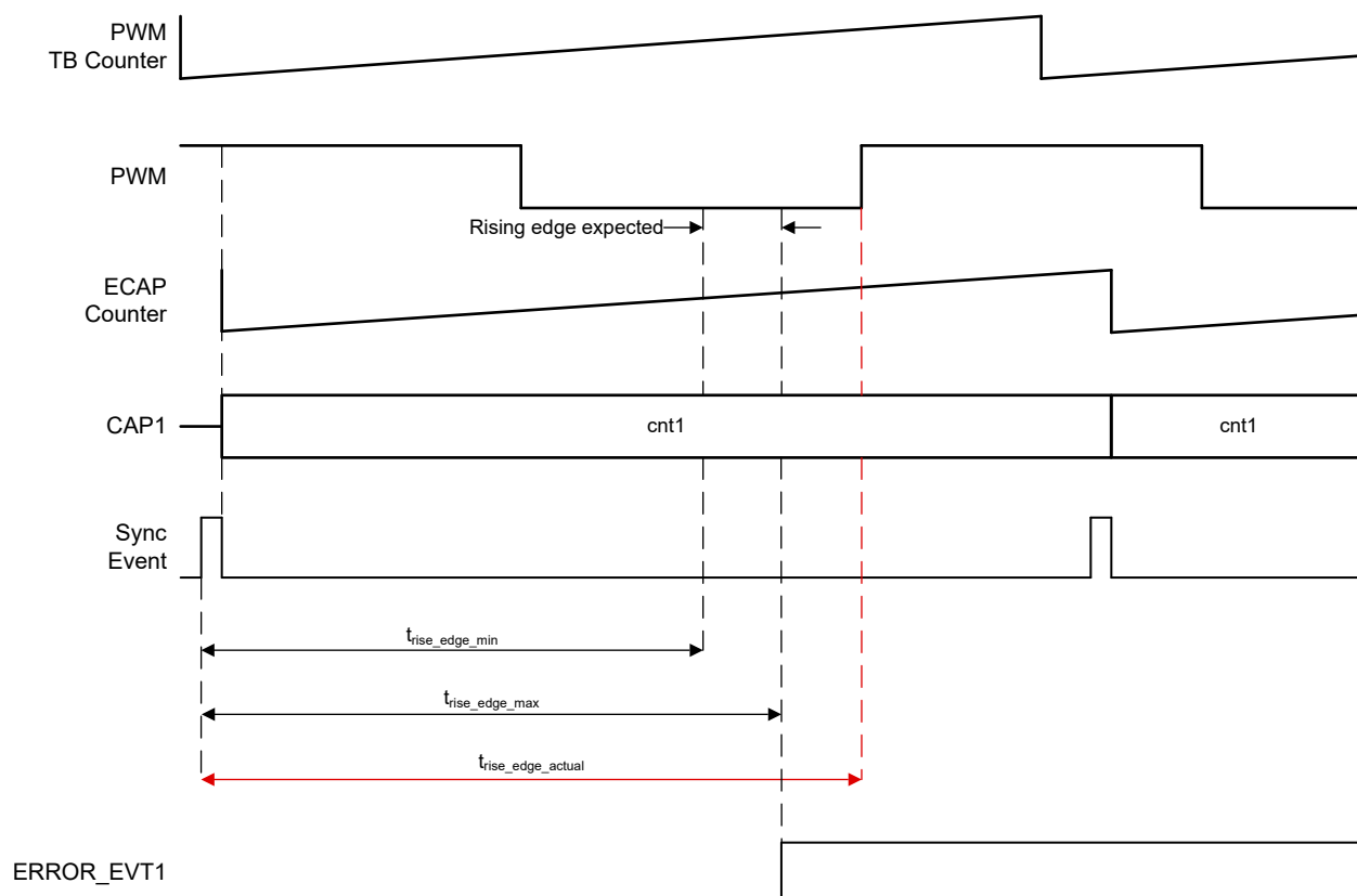
Figure 25-13. ECAP Signal Monitoring Unit Edge Error Example
