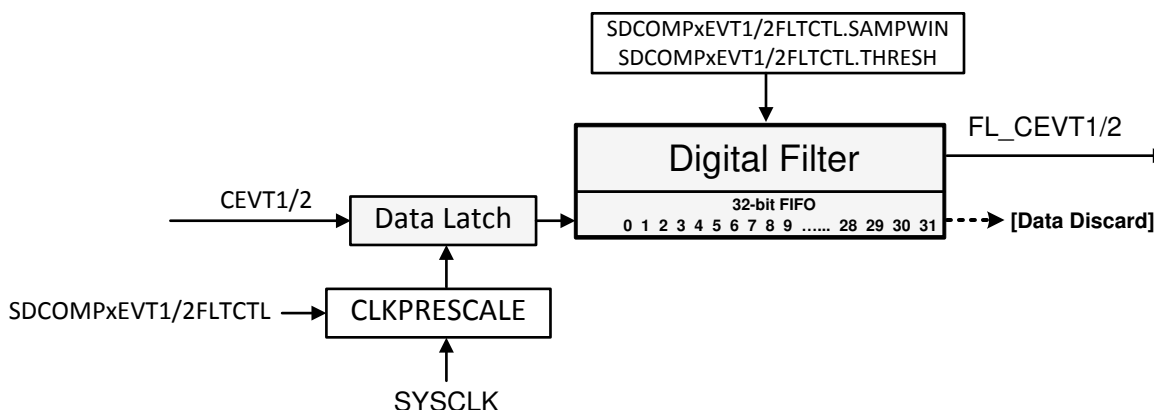
Figure 29-12. Digital Filter
