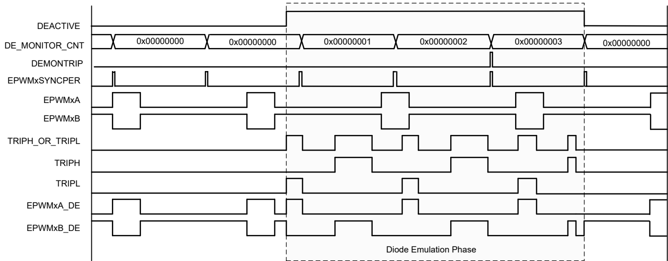
Figure 27-60. DE Mode Monitor Sequence
