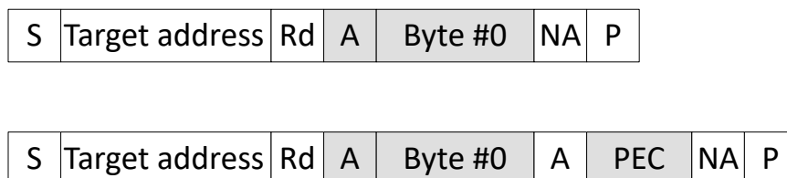
Figure 34-4. Receive Byte Message With and Without PEC
