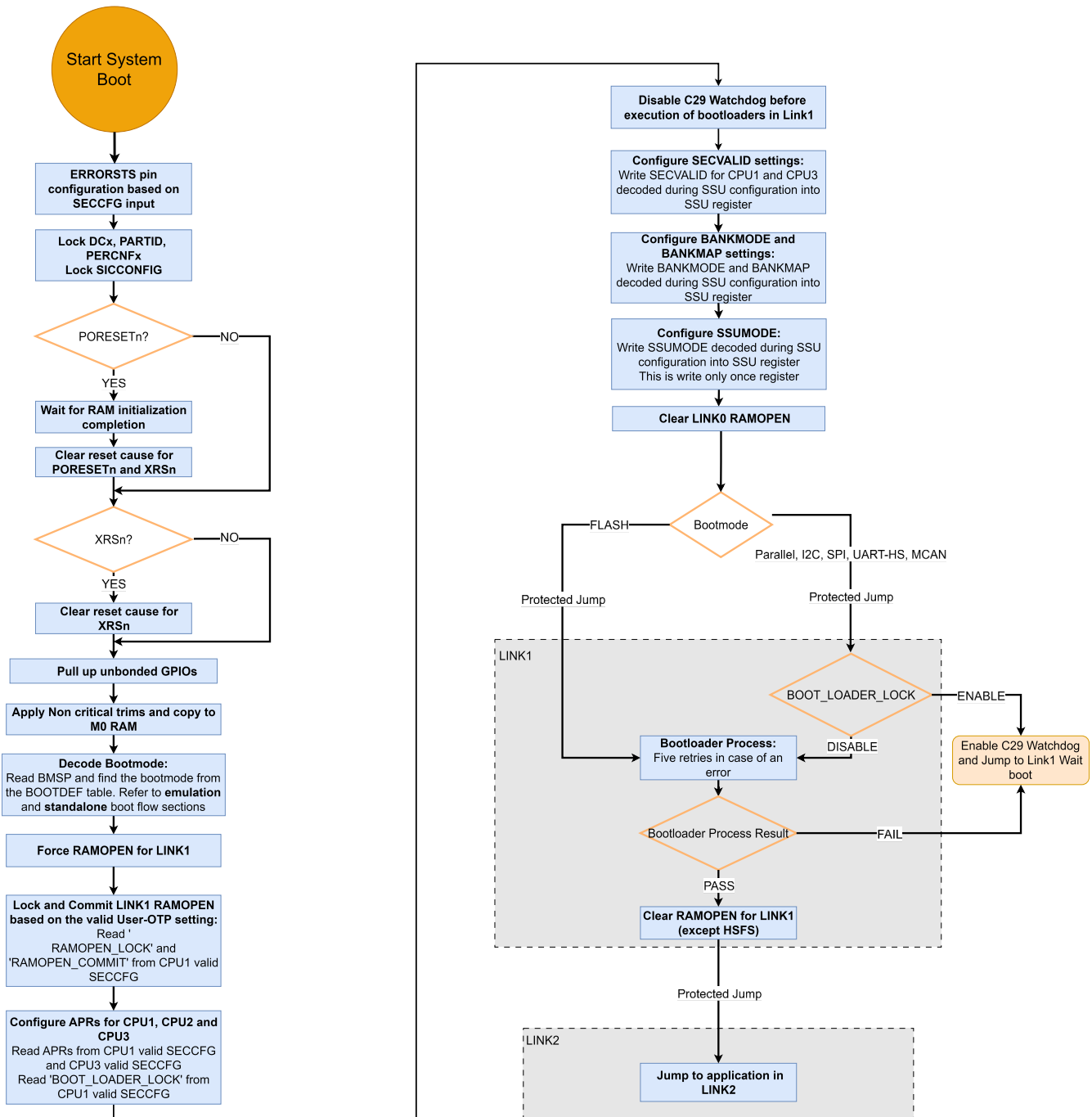
Figure 3-4. System Boot Flow to Application Code
