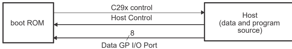
Figure 3-9. Overview of Parallel GPIO Bootloader Operation
