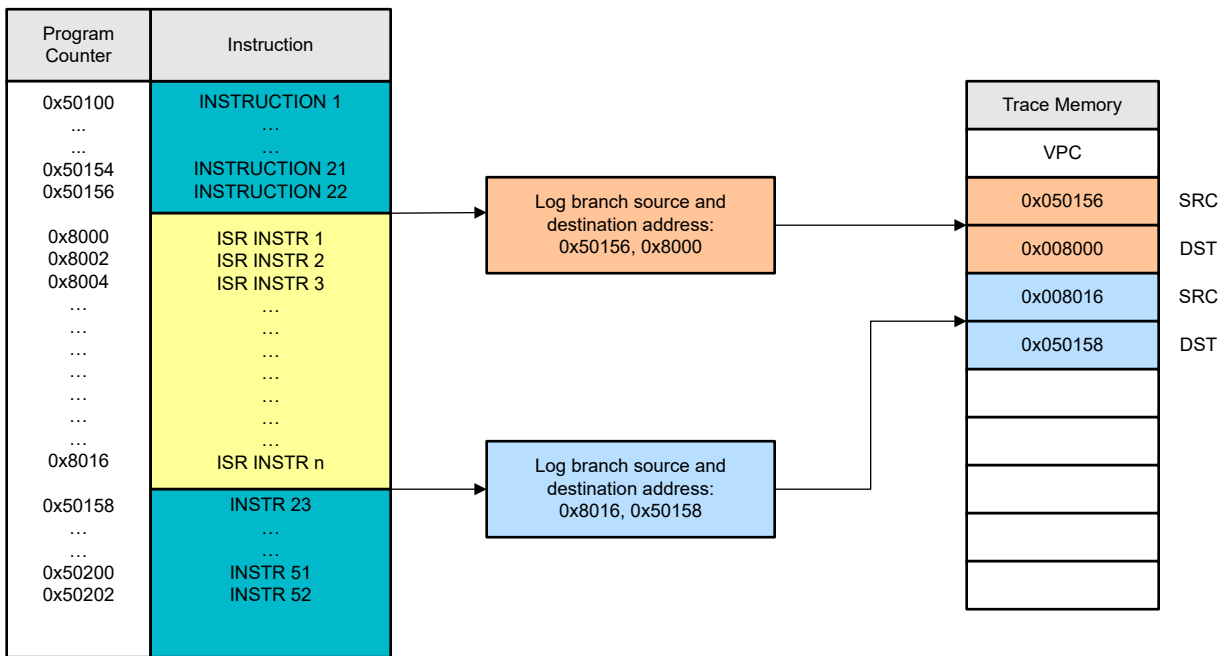
Figure 16-4. PC Trace Operation
