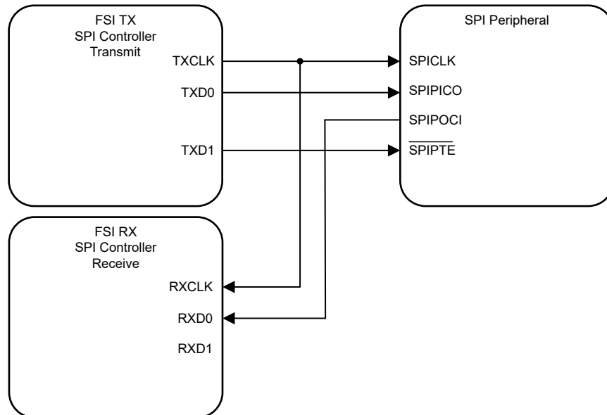
Figure 32-12. FSITX and FSIRX as SPI Controller, Full Duplex
