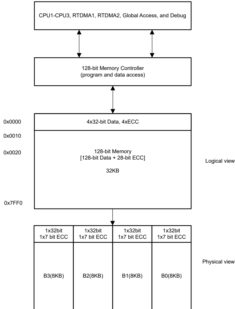
Figure 2-15. 128-Bit Memory
