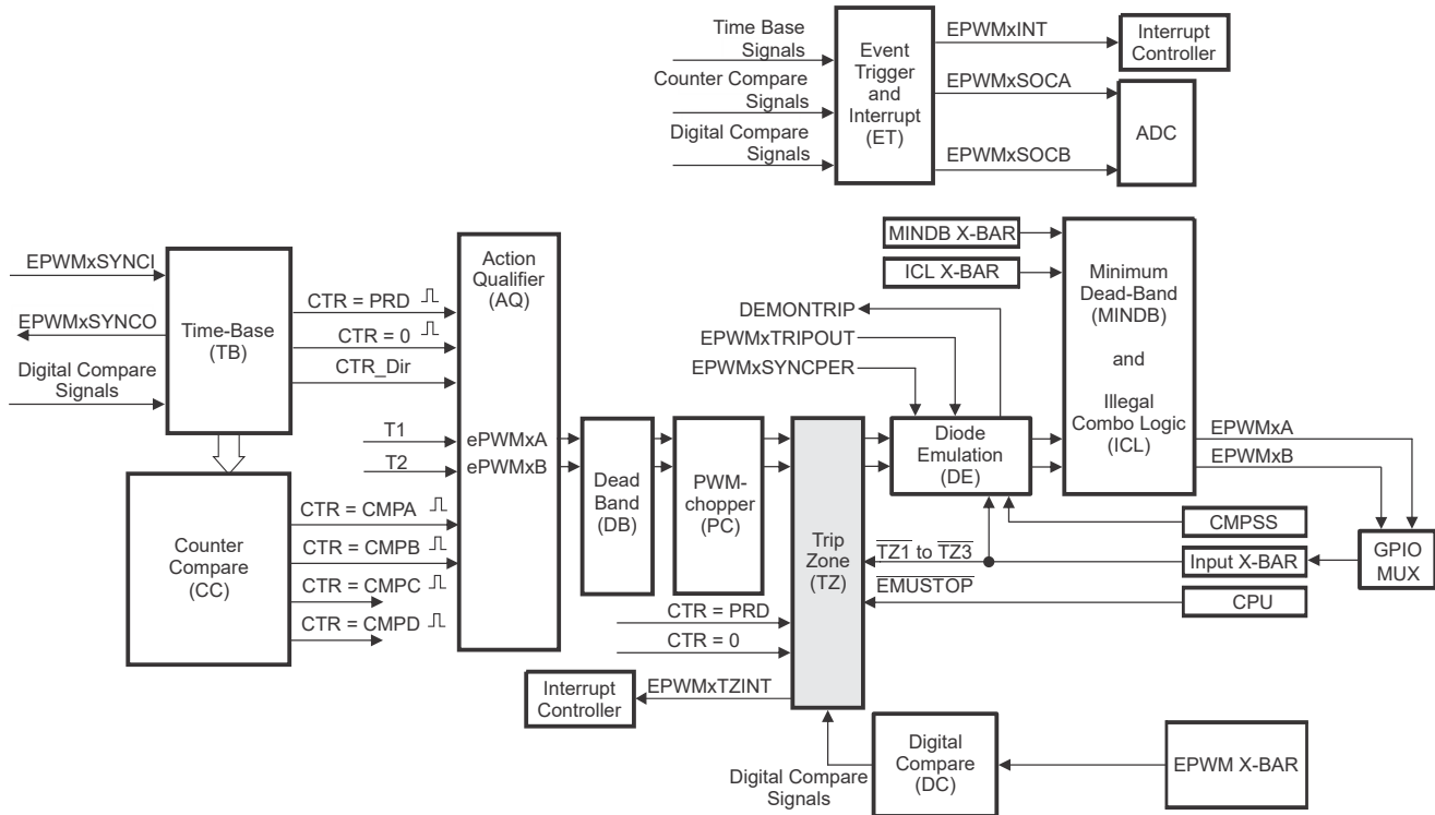
Figure 27-48. Trip-Zone Submodule
