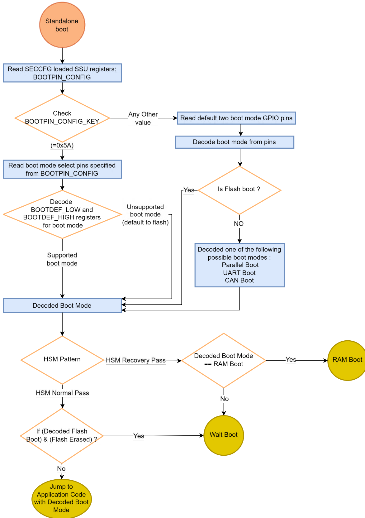
Figure 3-6. Standalone Boot Flow
