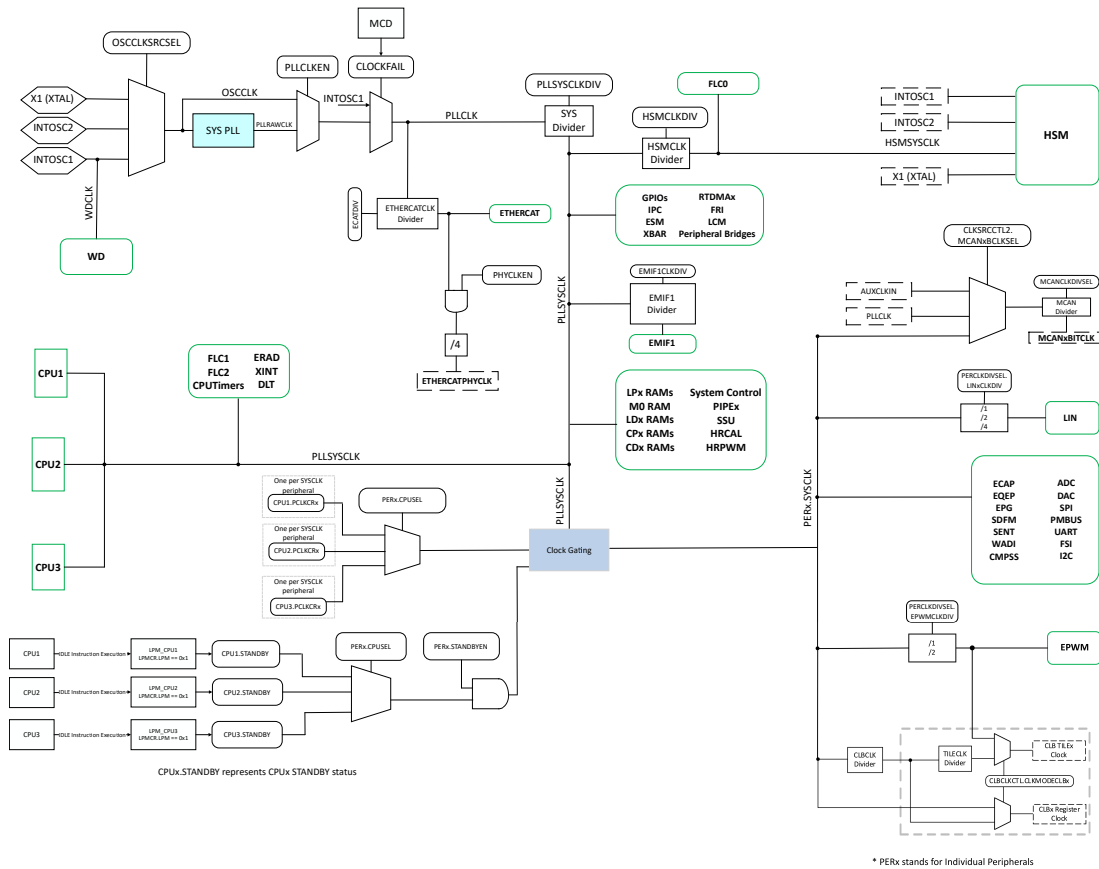
Figure 2-4. Clocking System
