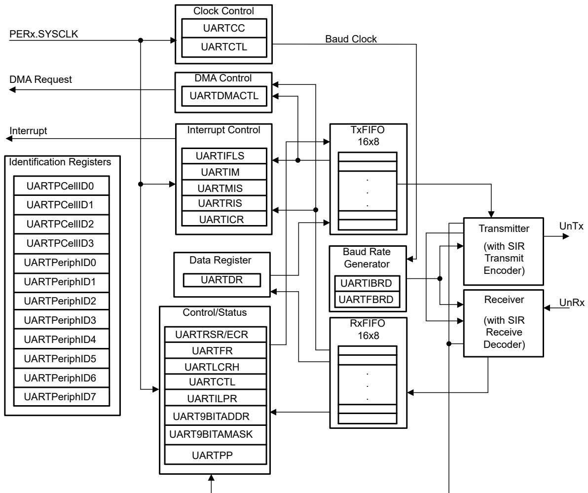
Figure 35-1. UART Module Block Diagram
