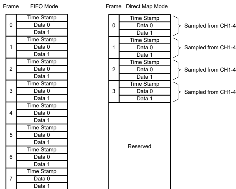
Figure 38-8. FIFO versus Direct Map Receive Modes
