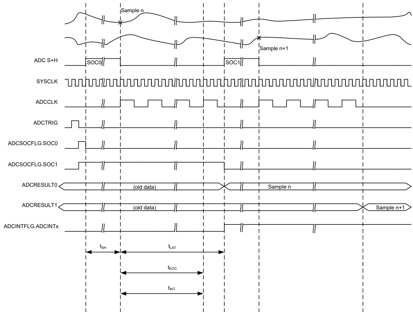
Figure 22-35. ADC Timings for 16-bit Mode in Late Interrupt Mode (SYSCLK Cycles)
