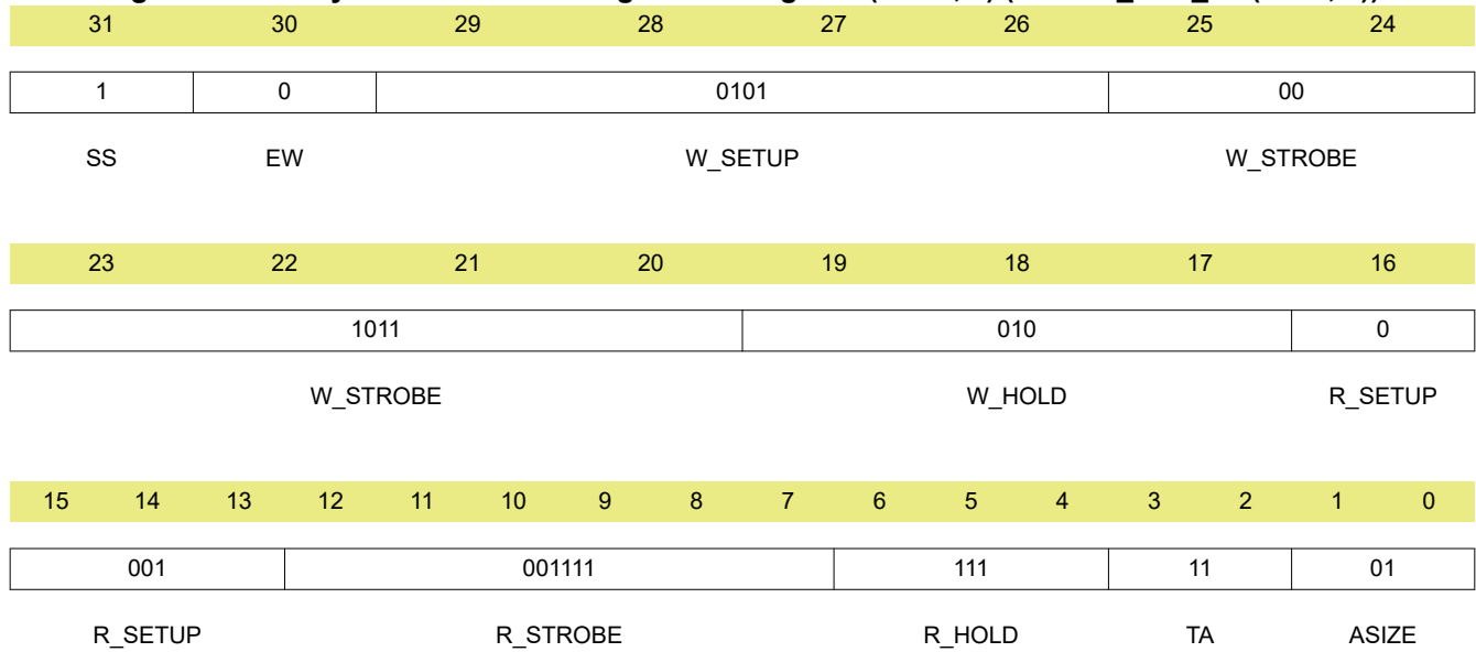
Figure 13-25. Asynchronous m Configuration Register ( m = 1, 2 ) (ASYNC_CS n _CR( n = 2, 3 ))
