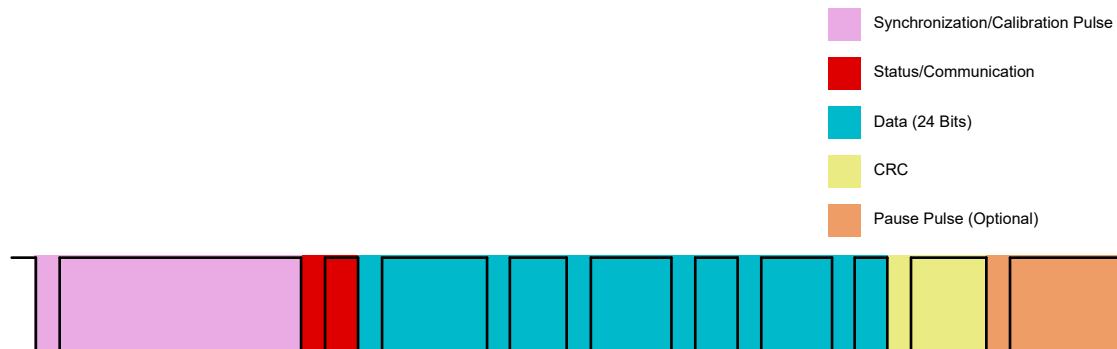
Figure 38-4. Fast Message
