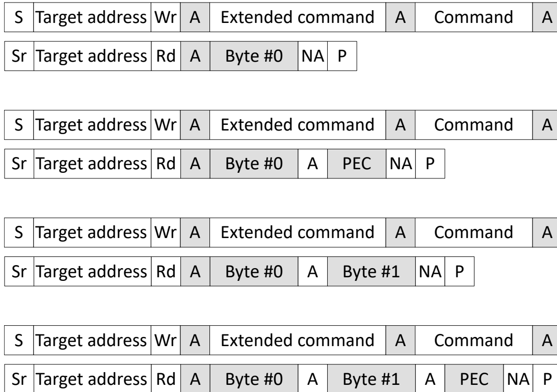
Figure 34-26. Extended Command Read Byte and Read Word Messages With and Without PEC
