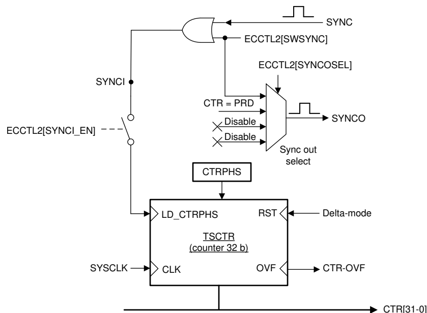
Figure 25-7. Details of the Counter and Synchronization Block
