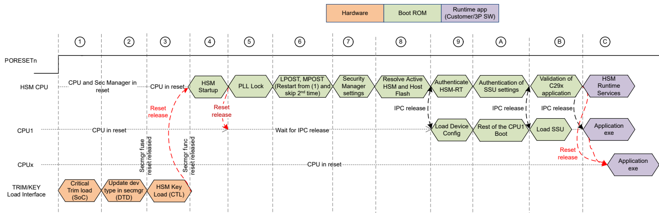
Figure 3-2. HS-SE Secure Boot Flow Diagram
