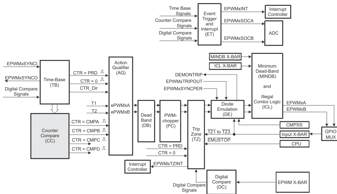
Figure 27-15. Counter-Compare Submodule
