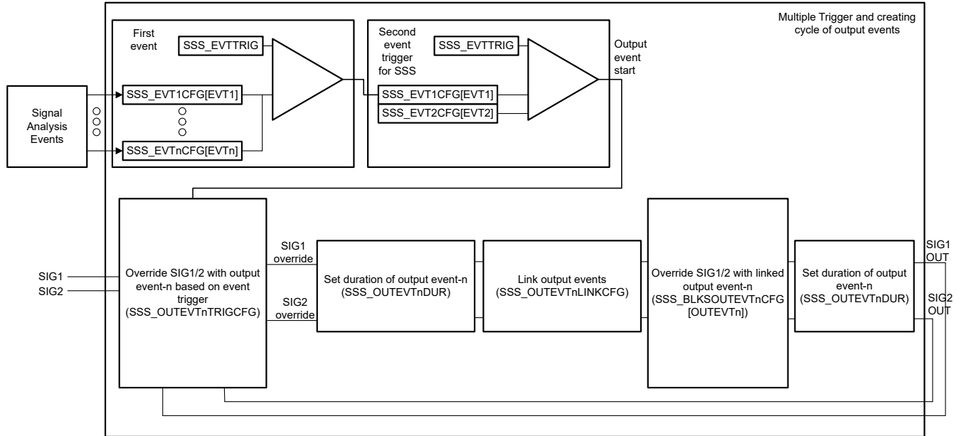
Figure 18-12. Multiple Trigger with Cyclic Pattern Output Events
