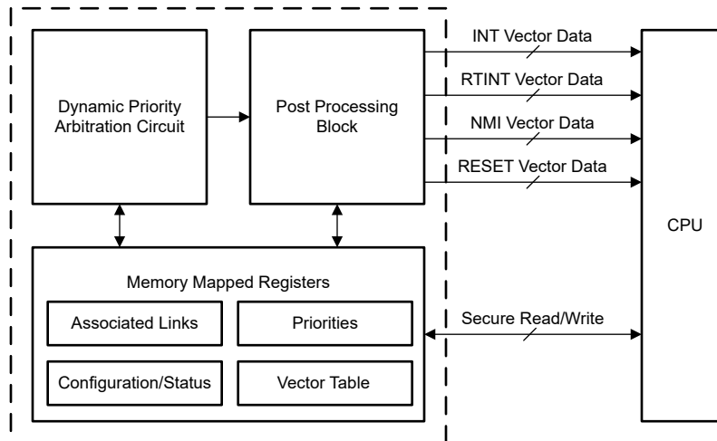
Figure 5-1. PIPE Architecture
