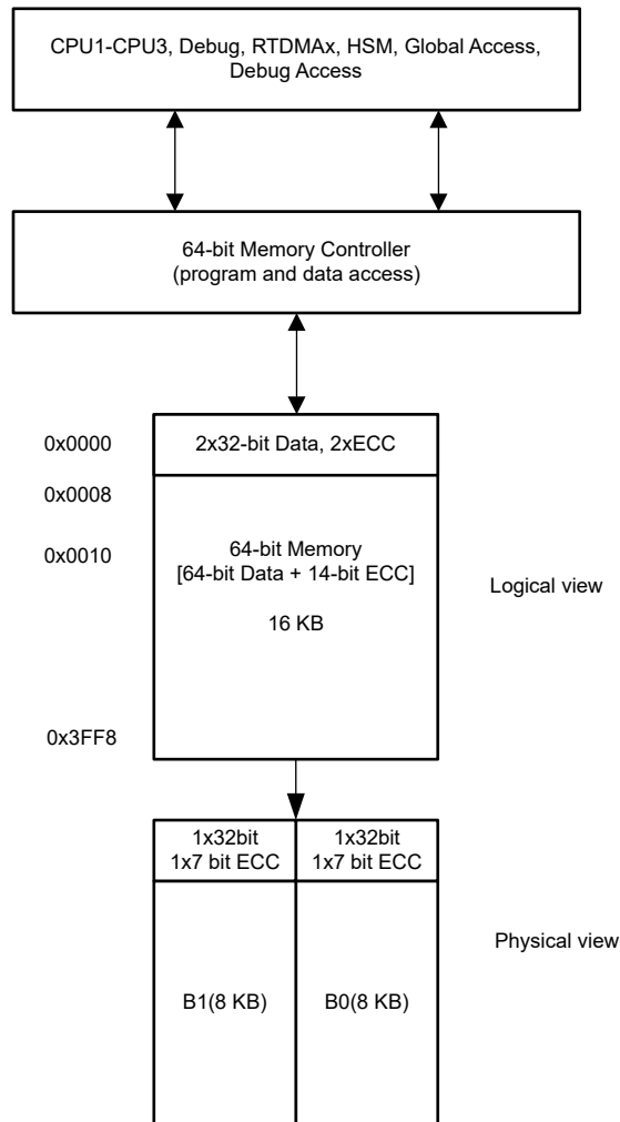
Figure 2-17. 64-Bit Memory
