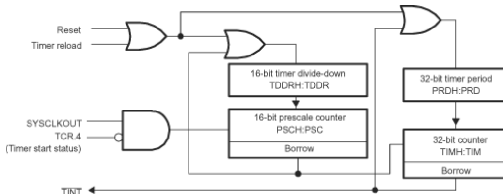
Figure 2-12. CPU Timers
