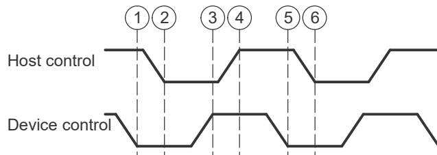
Figure 3-10. Parallel GPIO Bootloader Handshake Protocol
