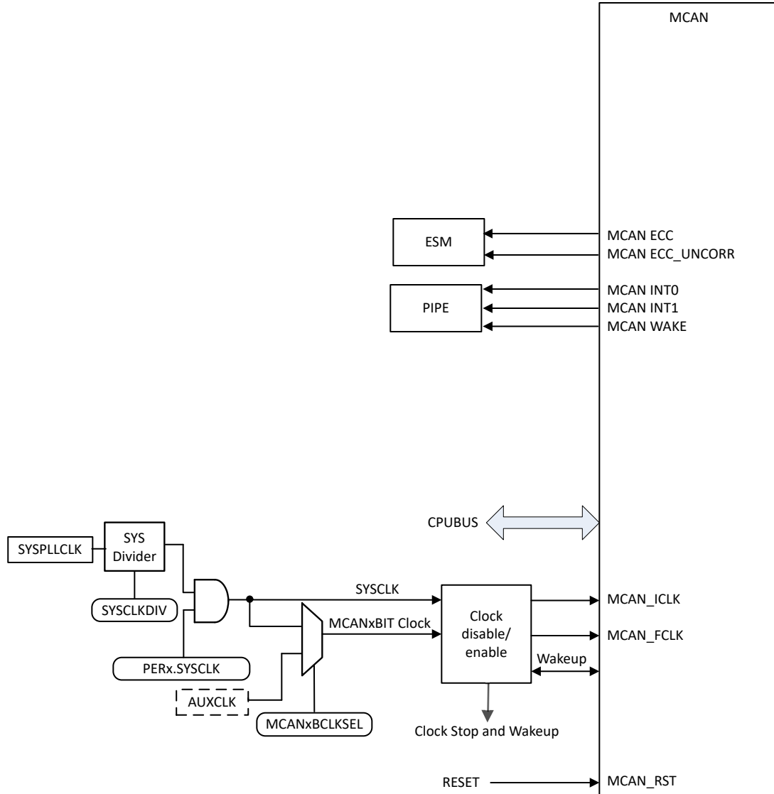
Figure 30-3. MCAN Integration
