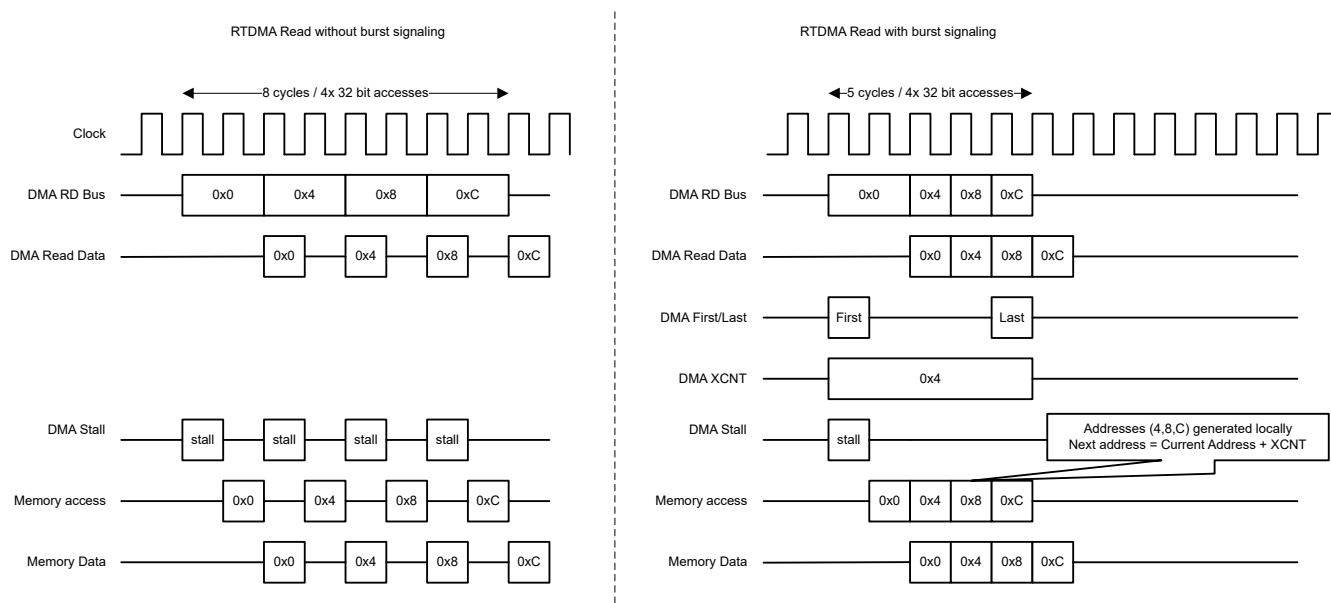
Figure 2-19. RTDMA Read
