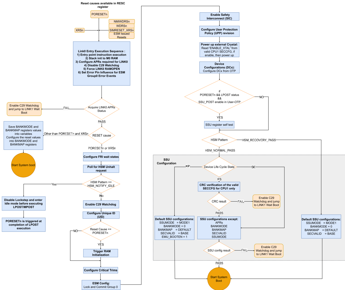
Figure 3-3. Device Boot Flow from Reset to System Boot
