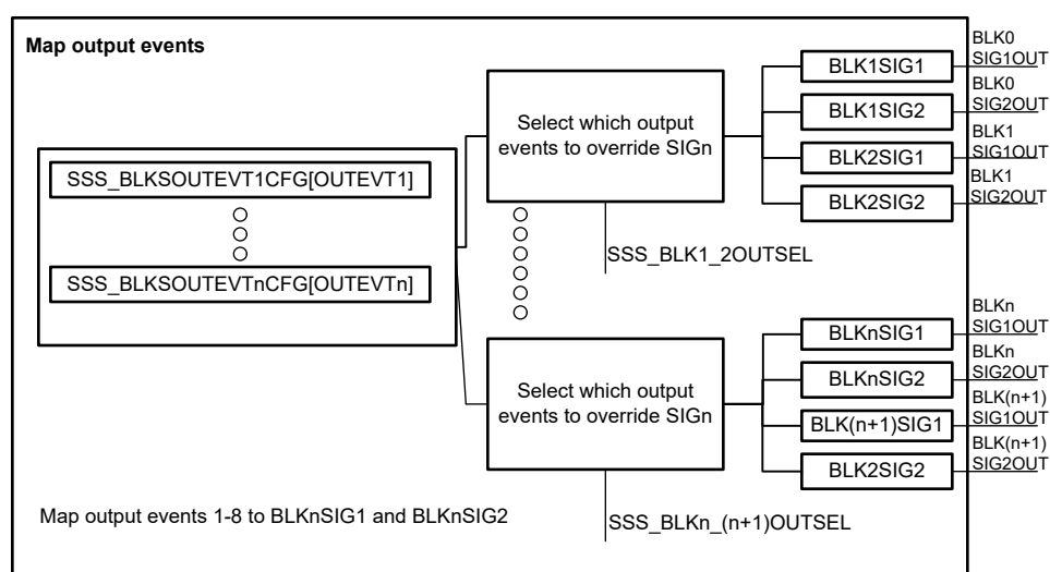
Figure 18-8. Map Output Events to BLK n SIG n
