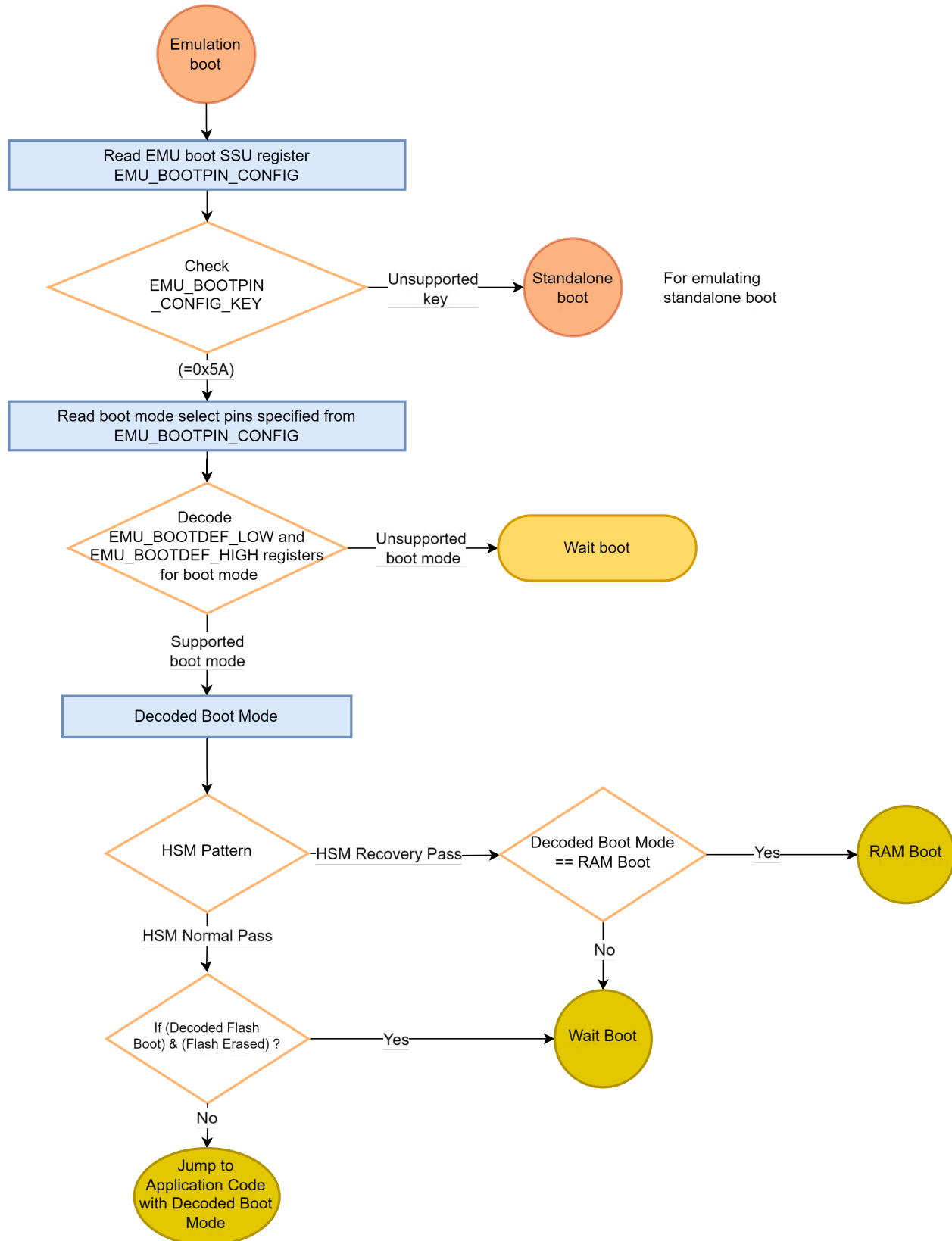
Figure 3-5. Emulation Boot Flow
