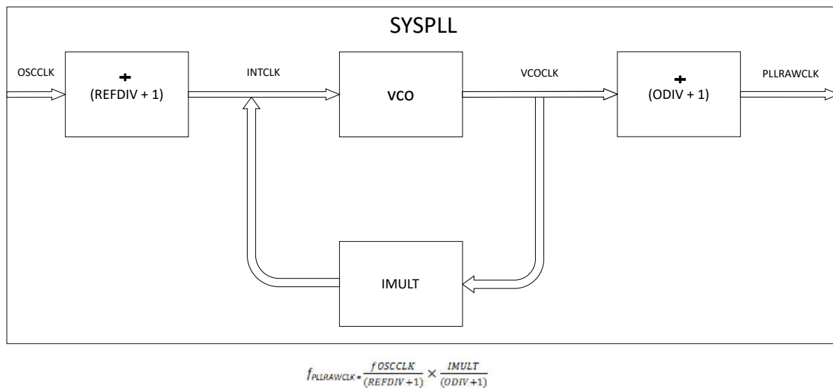
Figure 2-9. PLL
