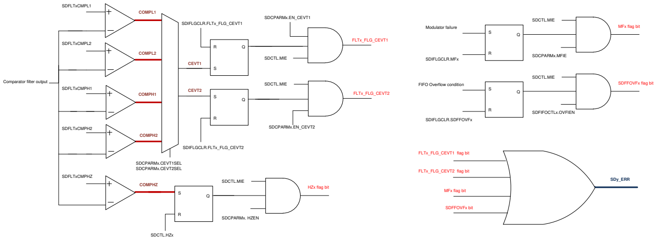
Figure 29-13. SDFM Error (SD_ERR) Interrupt Sources
