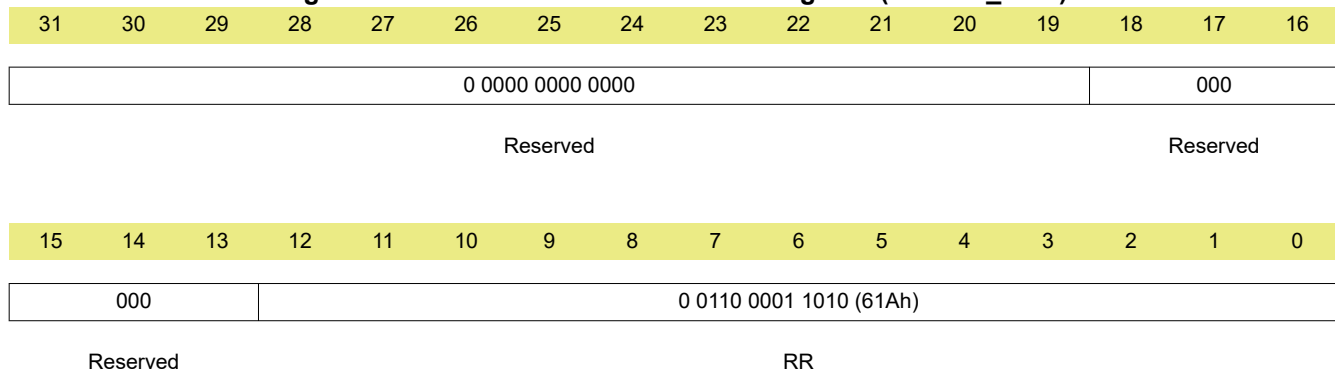
Figure 13-21. SDRAM Refresh Control Register (SDRAM_RCR)
