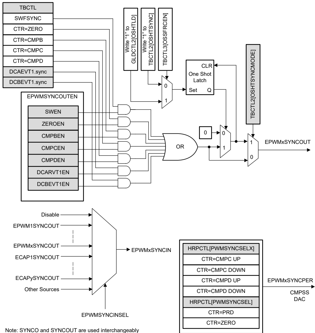
Figure 27-7. Time-Base Counter Synchronization Scheme
