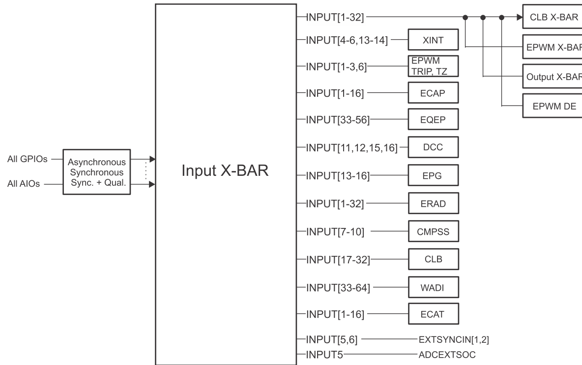
Figure 19-1. Input X-BAR
