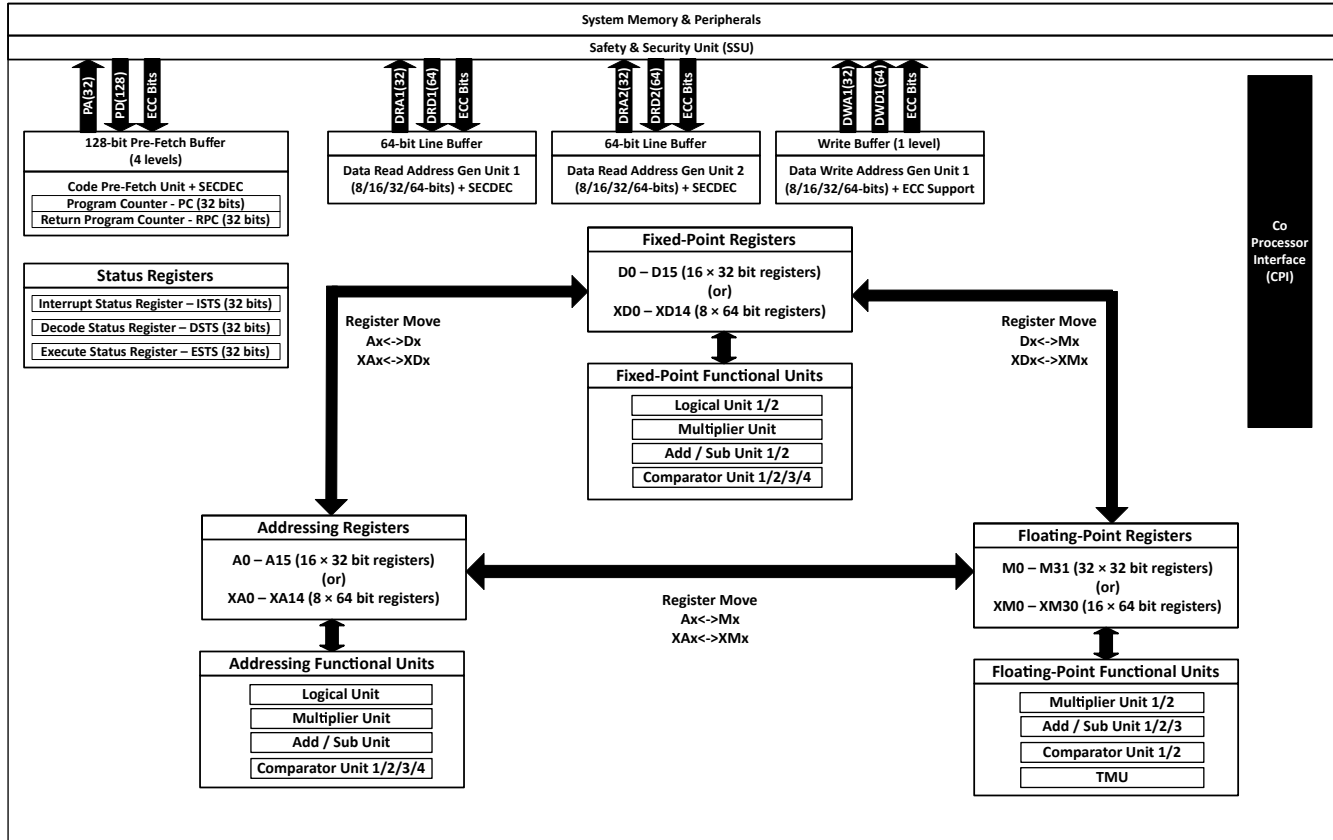
Figure 1-1. CPU Architecture Block Diagram
