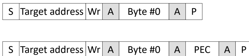
Figure 34-3. Send Byte Message With and Without PEC
