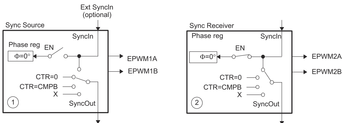
Figure 27-89. EPWM1 Configured as a Typical Sync Source, EPWM2 Configured as a Sync Receiver
