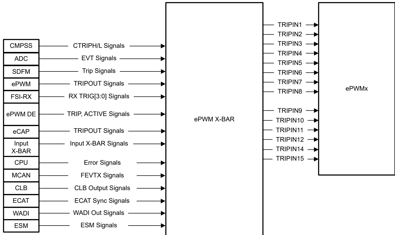
Figure 27-87. ePWM X-BAR
