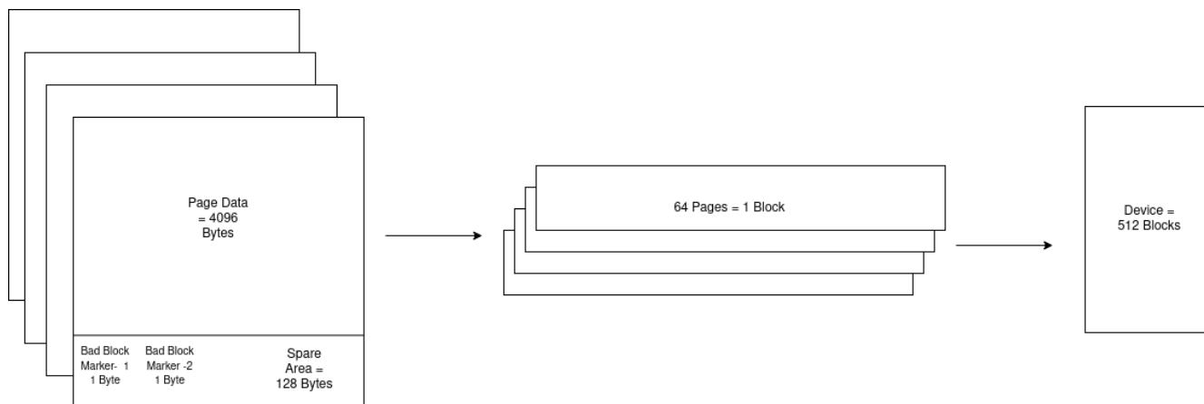
Figure 2-1. Flash Memory Architecture for W35N01JW Winbond Flash
