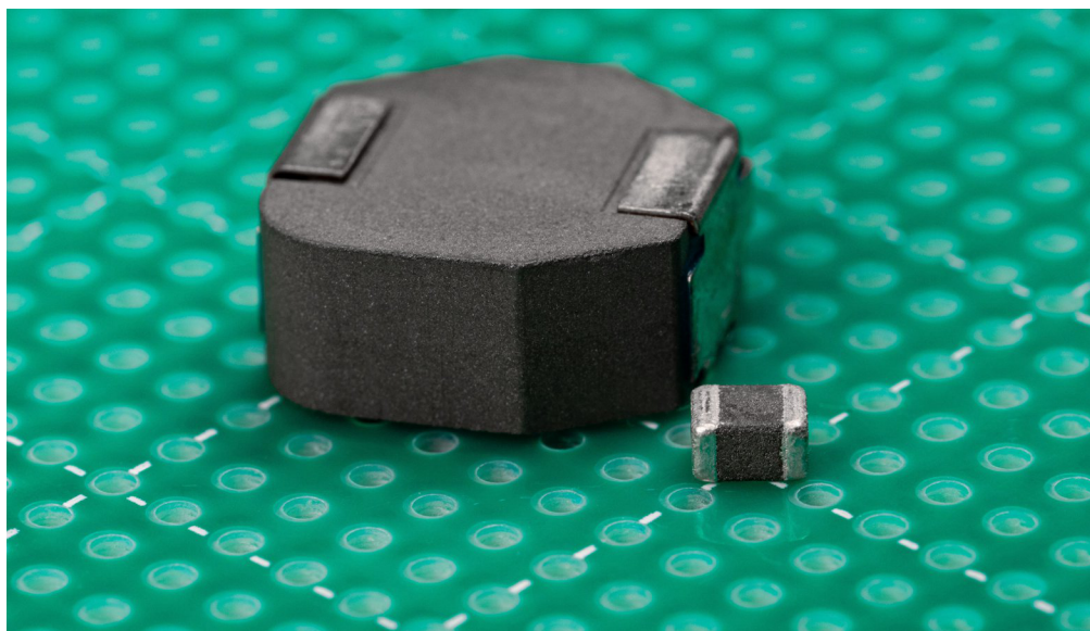
Figure 1. Size comparison of an 8.2μH inductor (400kHz) and a tiny 3.3μH inductor (2.1MHz)
