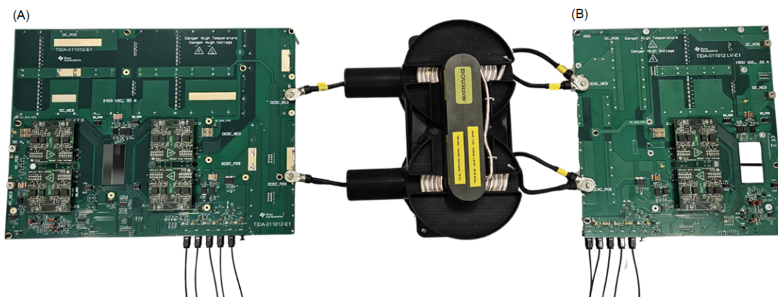
Figure 5. A 5050kW SiC-based modular SST, with a plastic optical fiber interface between medium-voltage (A) and low-voltage (B) PCBs
