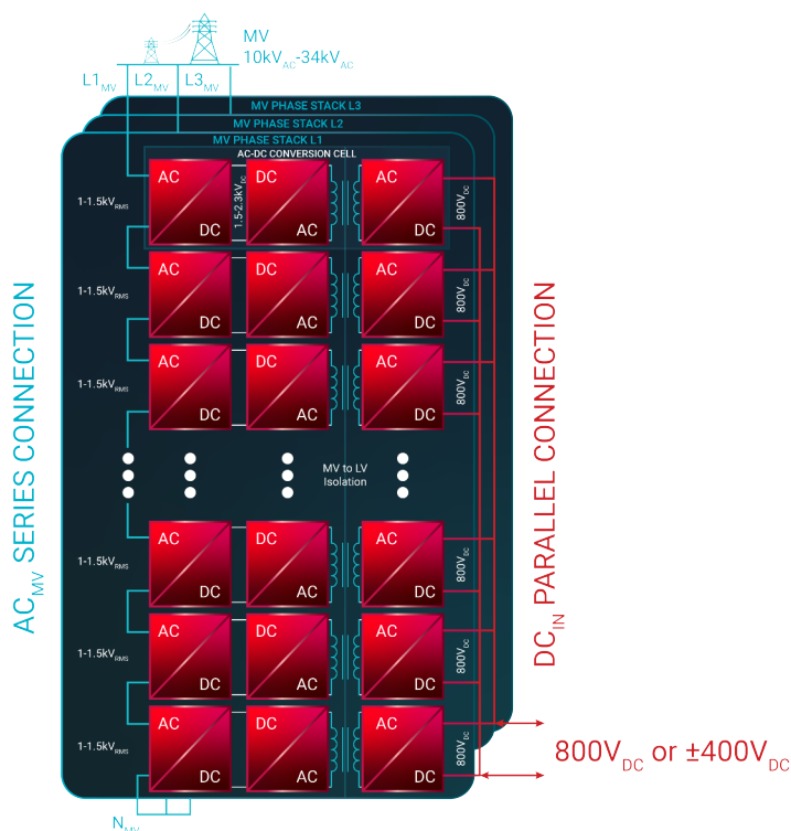
Figure 2. A typical SST implementation, with stacked air conditioning and mechanical ventilation converters and parallel low-voltage outputs
