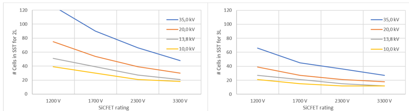
Figure 3. Cell scaling for 2L and 3L conversion cells based on SiC rating
