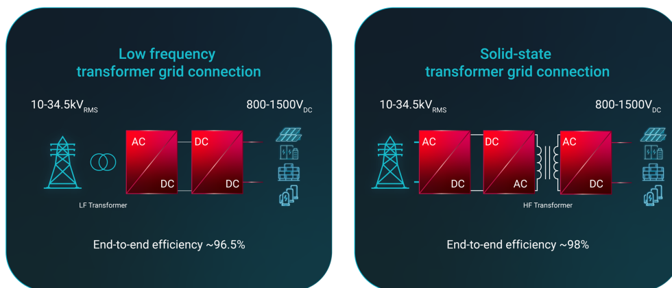
Figure 1. Efficiency savings with a low-frequency transformer-based grid connection vs an SST implementation
