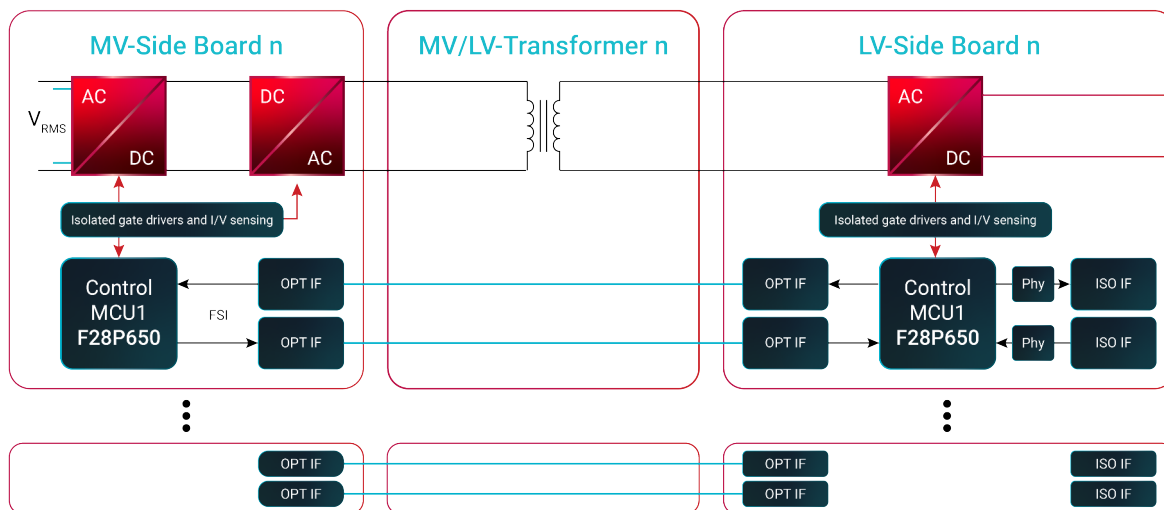
Figure 4. Conversion cell architecture with AC/DC and isolated DC/DC
