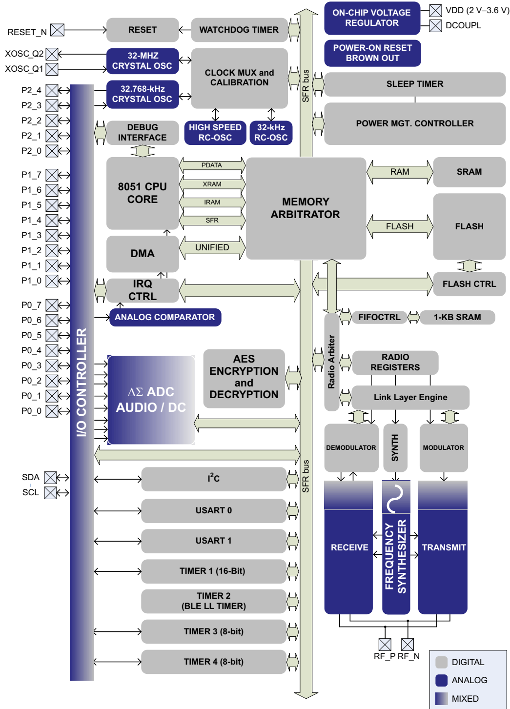
Figure 1. Block Diagram
