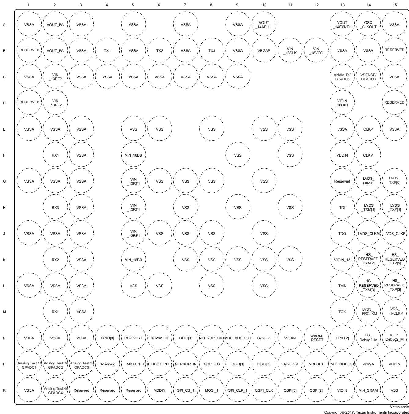
Figure 7-1. Pin Diagram
