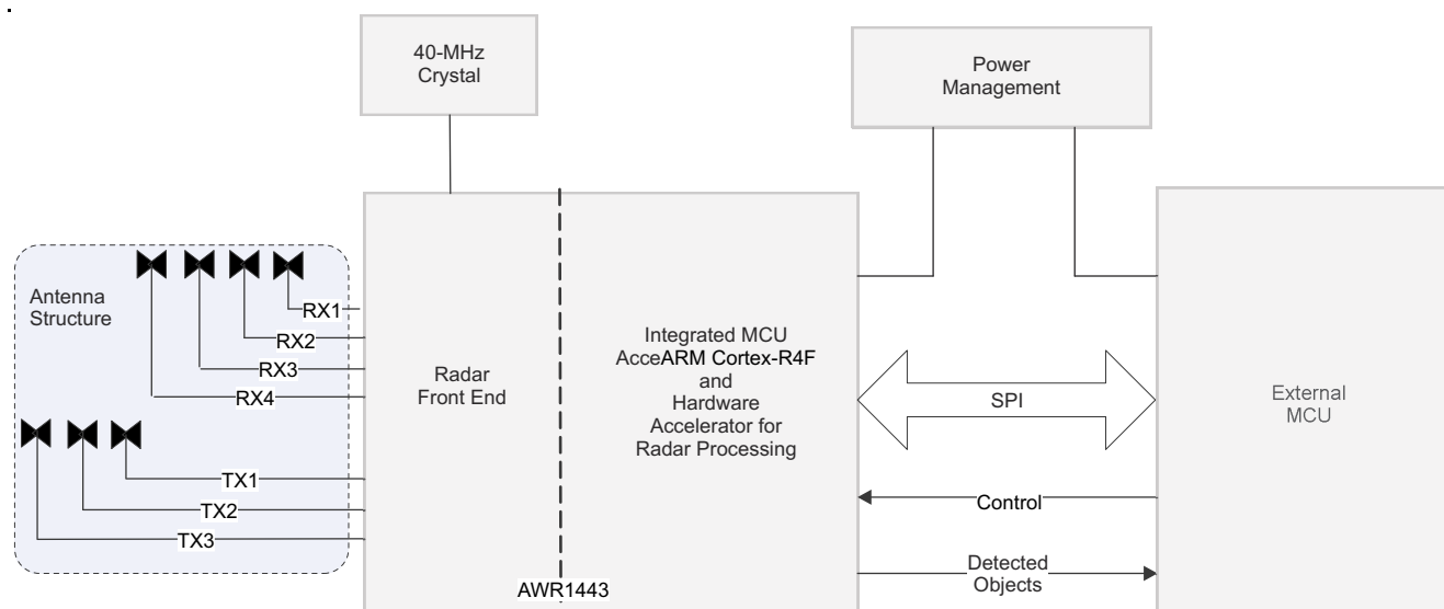
Figure 10-1. Short-Range Radar
