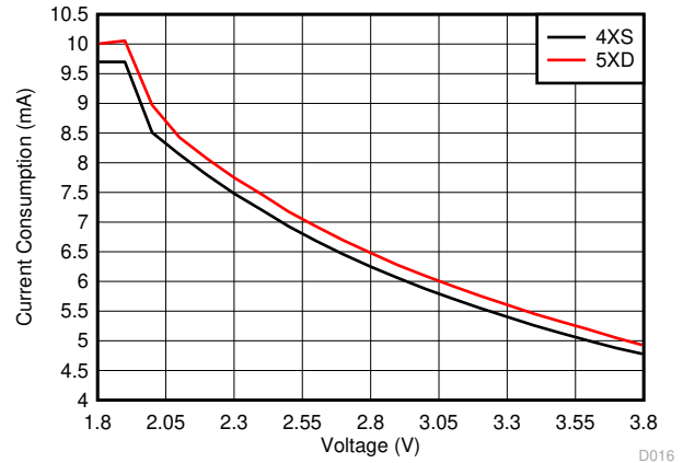
Figure 8-11. RX Mode Current Consumption vs Supply Voltage (VDD5)
