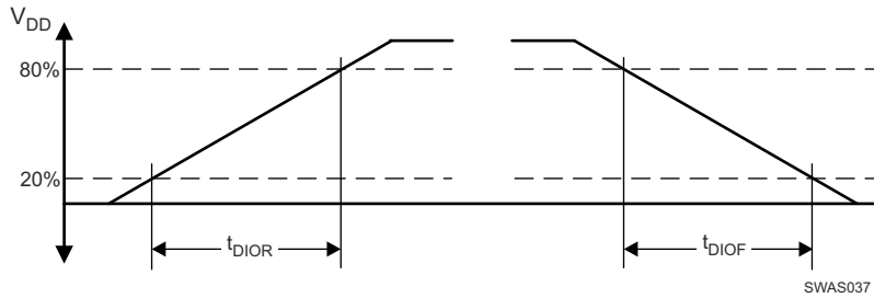
Figure 7-15. DIO Timing Diagram
