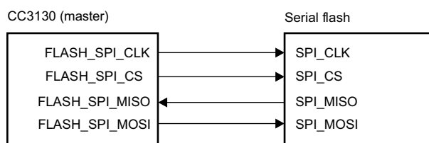
Figure 7-16. SPI Flash Interface
