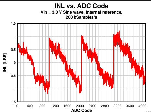
Figure 8-25. INL vs. ADC Code
