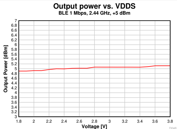
Figure 8-20. Output Power vs. Supply Voltage (VDD) (BLE 1 Mbps, 2.44 GHz, +5 dBm)
