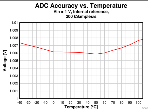
Figure 8-27. ADC Accuracy vs. Temperature
