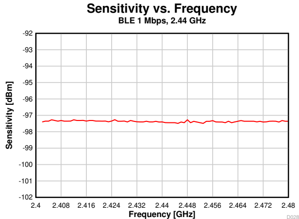
Figure 8-10. Sensitivity vs. Frequency (BLE 1 Mbps, 2.44 GHz)
