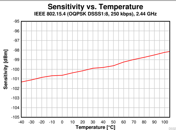
Figure 8-13. Sensitivity vs. Temperature (250 kbps, 2.44 GHz)
