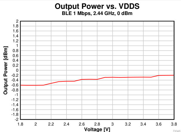
Figure 8-19. Output Power vs. Supply Voltage (VDD) (BLE 1 Mbps, 2.44 GHz)
