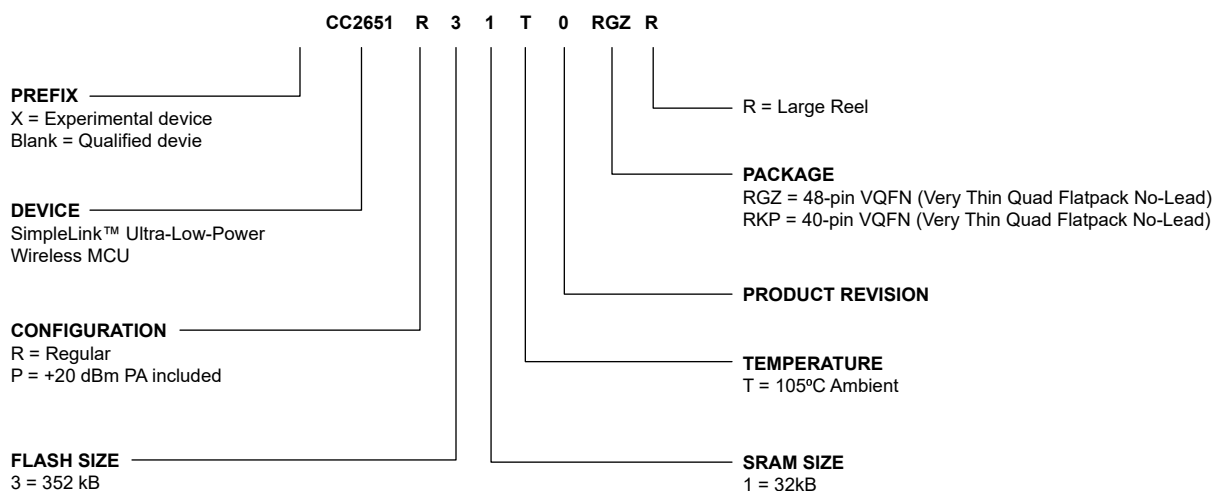
Figure 11-1. Device Nomenclature
