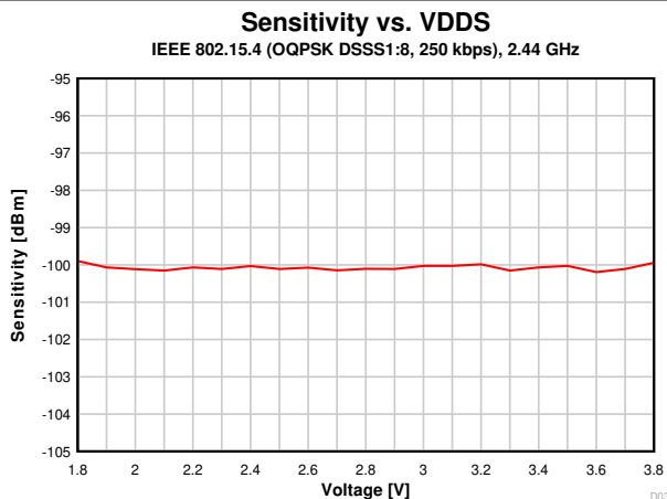
Figure 8-16. Sensitivity vs. Supply Voltage (VDDS) (250 kbps, 2.44 GHz)
