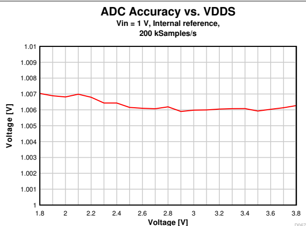
Figure 8-28. ADC Accuracy vs. Supply Voltage (VDD)
