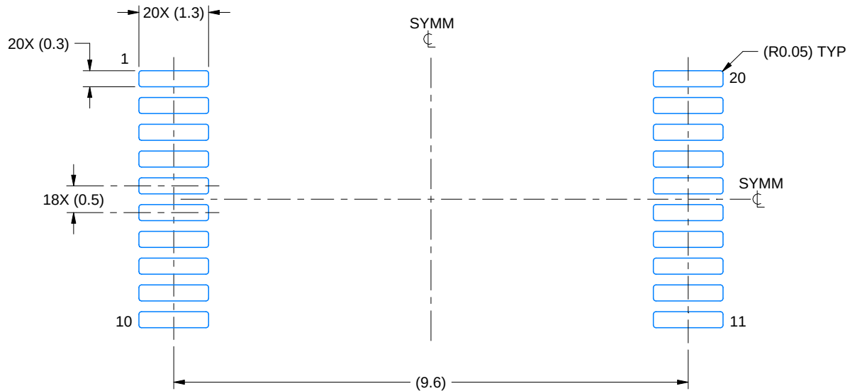
LAND PATTERN EXAMPLE EXPOSED METAL SHOWN SCALE: 10X
