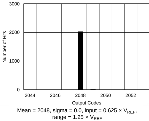
Figure 10. DC Histogram for Mid-Scale Inputs ( 1.25 \times V_{REF} )
