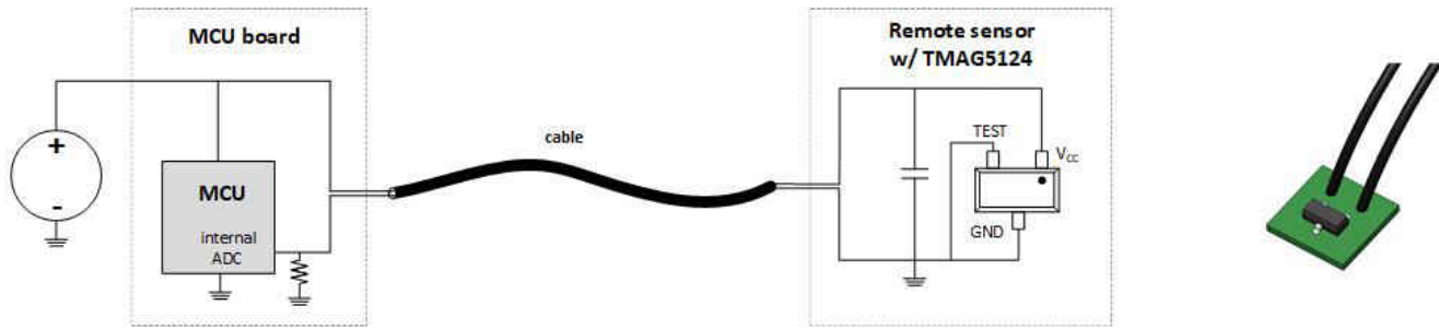
Figure 3. TMAG5124 Two-Wire Connection and Small PCB Implementation
