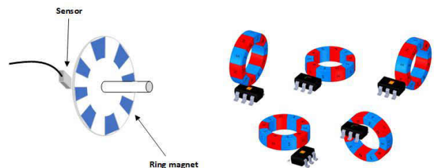
Figure 1. Rotary Encoding Using Ring Magnets, and Various Sensor Placements
