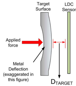
Figure 2. Inductive Sensing Technology for Touch Buttons
