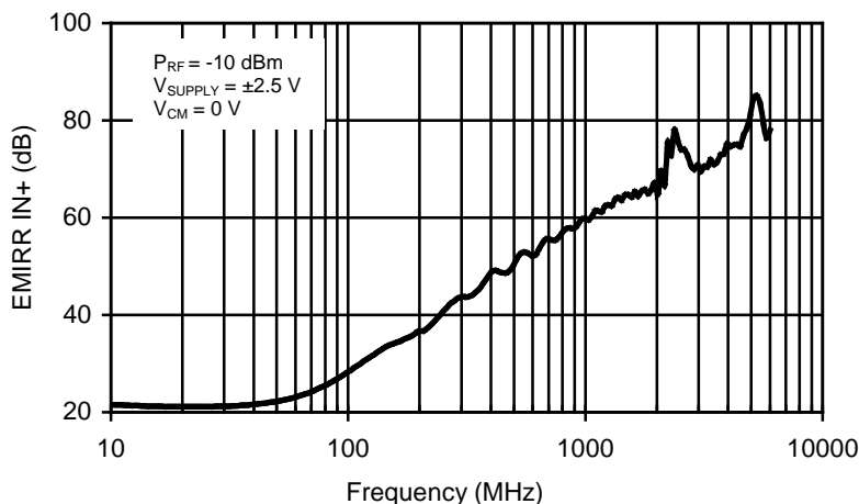
Figure 1. TLC2252 EMIRR IN+ vs Frequency
