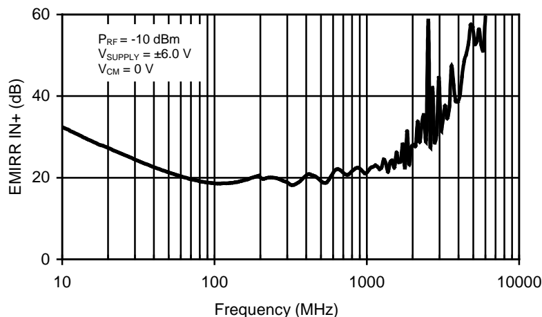
Figure 1. TLV2371 EMIRR IN+ vs Frequency
