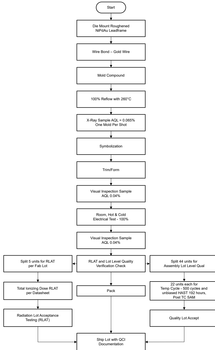
Figure 1-1. CDCLVP111-SEP Space Enhanced Plastic Production Flow Chart
