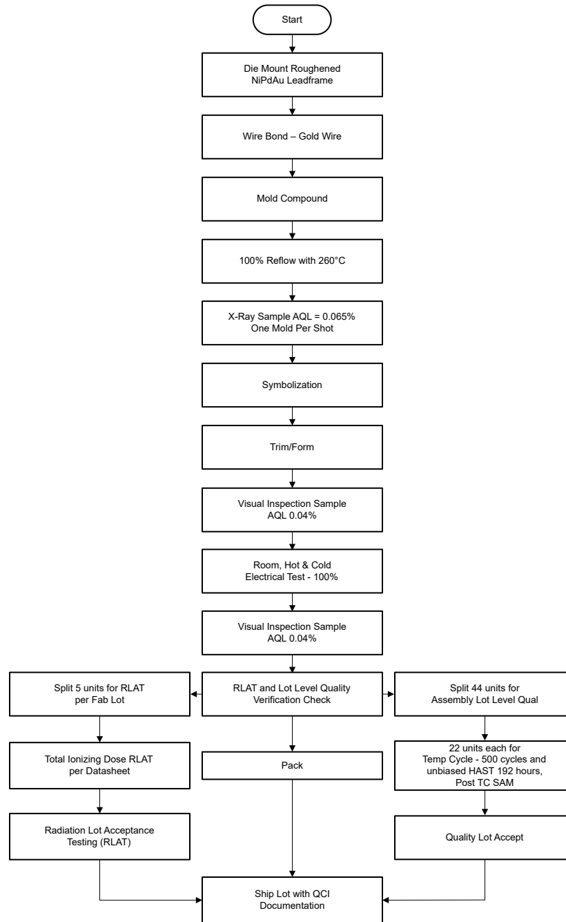
Figure 1-1. TPS7H1121-SEP Space Enhanced Plastic Production Flow Chart
