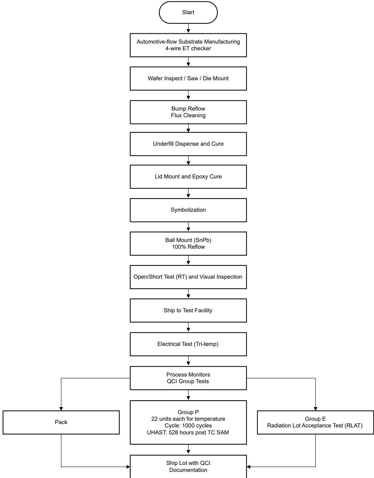
Figure 1-1. DAC39RF10-SEP Space Enhanced Plastic Production Flow Chart
