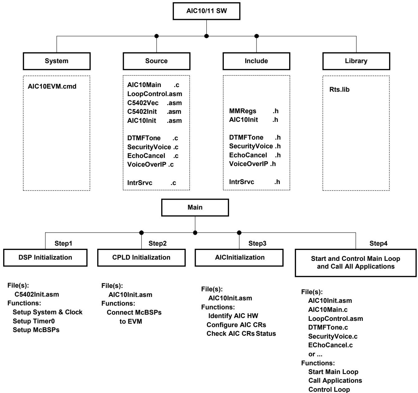
Figure 10. Software Tree Structure
