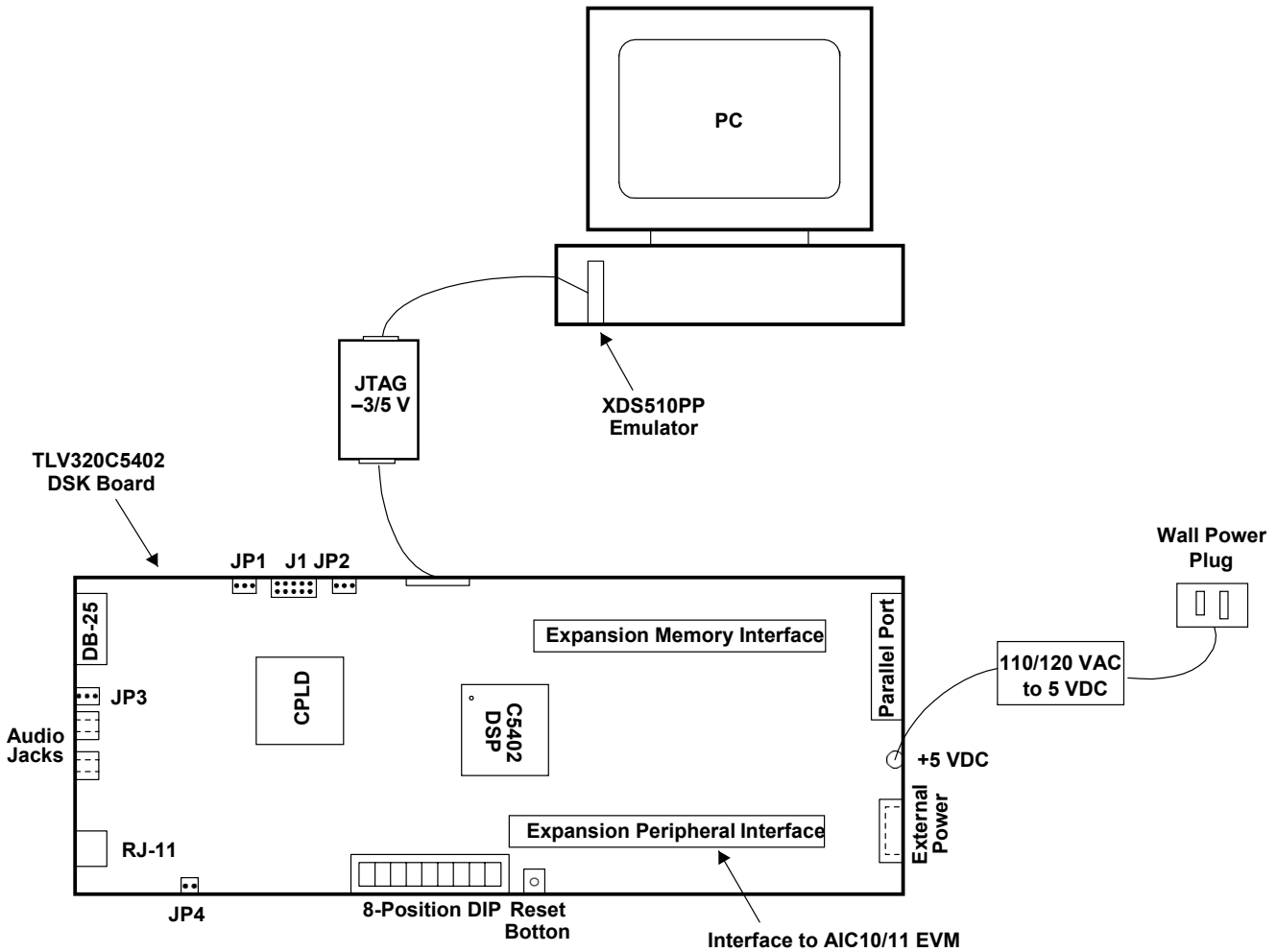
Figure 2. System Connection
