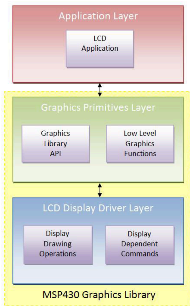
Figure 2-2. System Overview Stack Diagram
