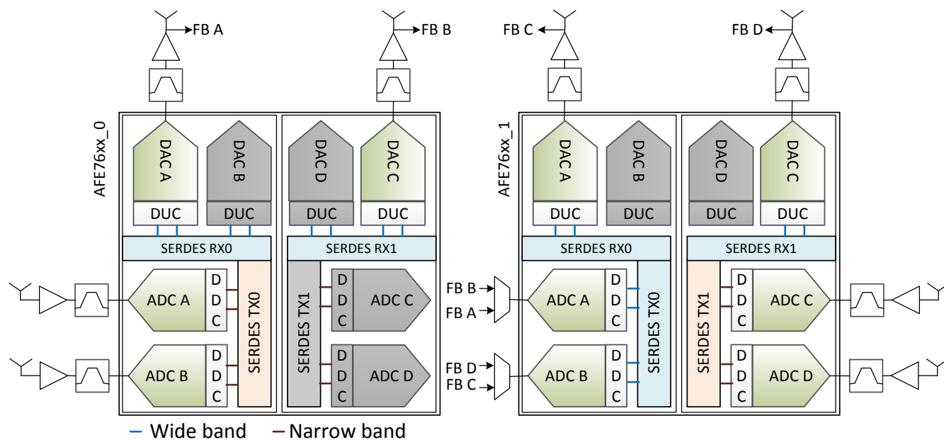
Figure 3-3. 4T4R2FB System Case 1
