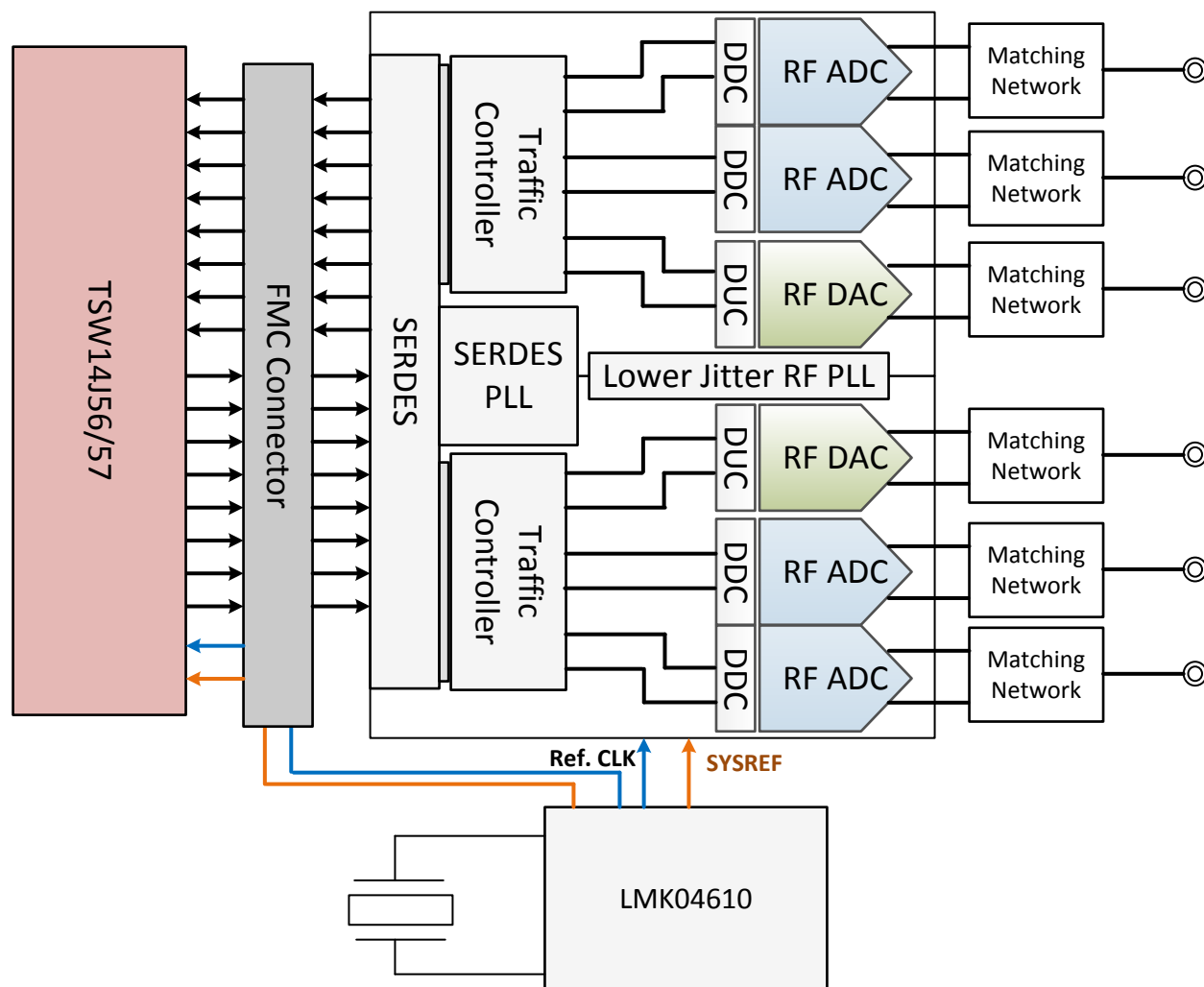
Figure 2-2. TSW4086 EVM Test Setup
