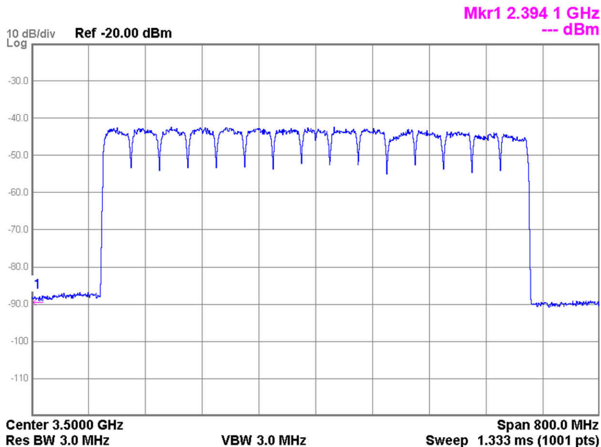
Figure 6-6. TX Path Output with Wideband Signal (600MHz)
