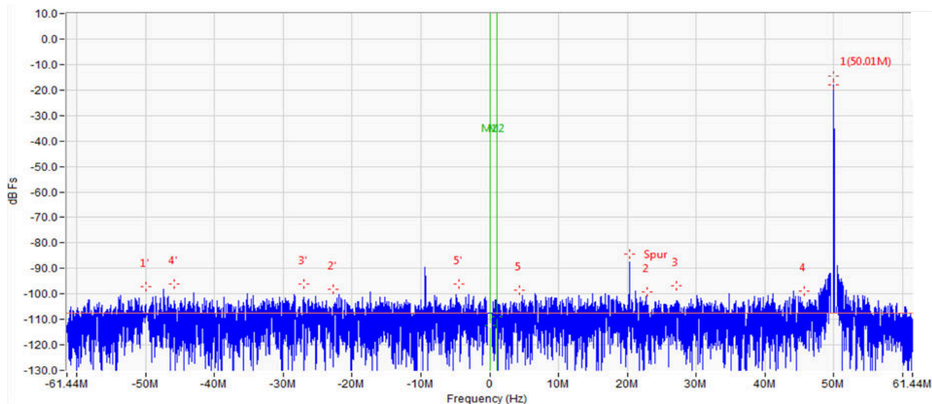
Figure 6-1. RX Path Output with Single Tone at 1750MHz, -15dBFS
