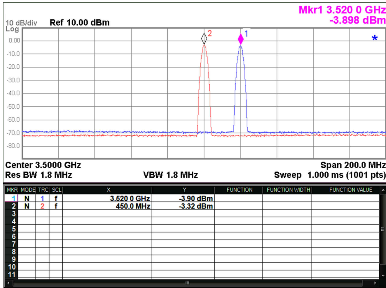
Figure 6-5. Digital RX-to-TX Direct Loopback : RX input - CW at 450MHz, TX output at 3520MHz
