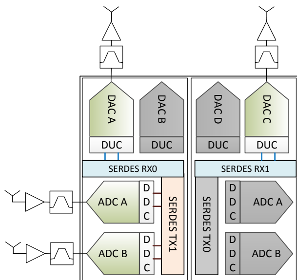
Figure 3-1. 2T2R Configuration
