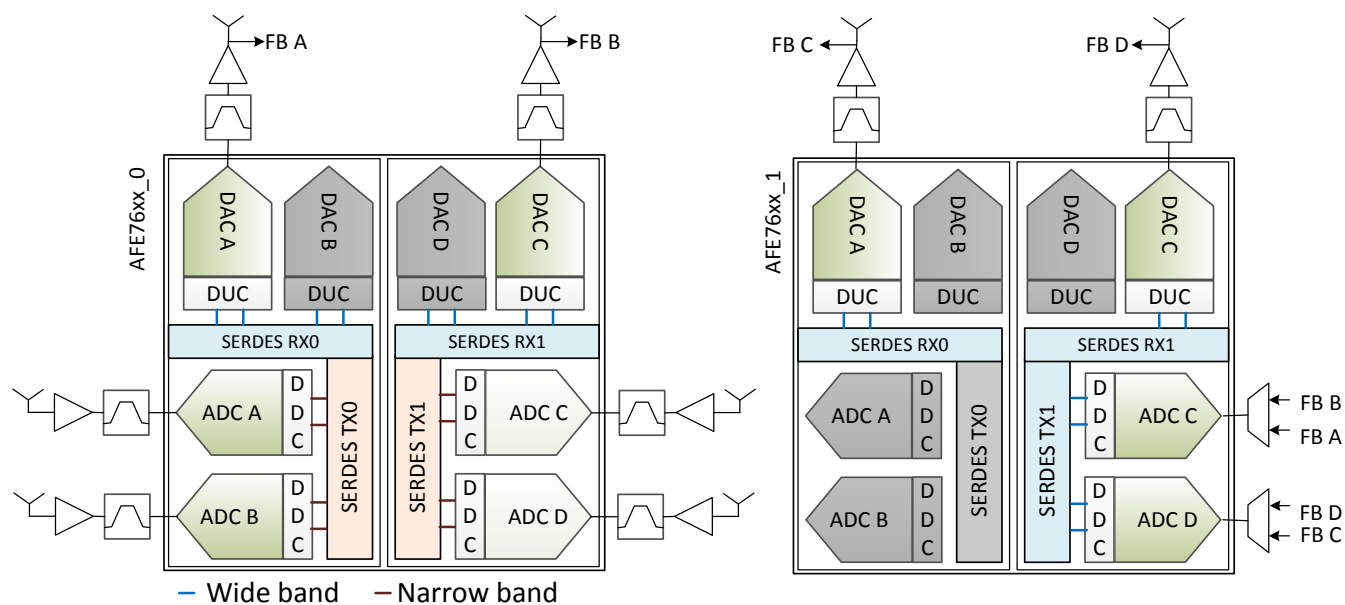
Figure 3-4. 4T4R2FB System Case 2
