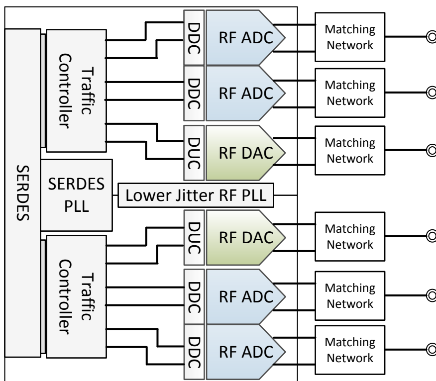
Figure 1-1. AFE76xx with Integrated RF sampling ADCs and DACs
