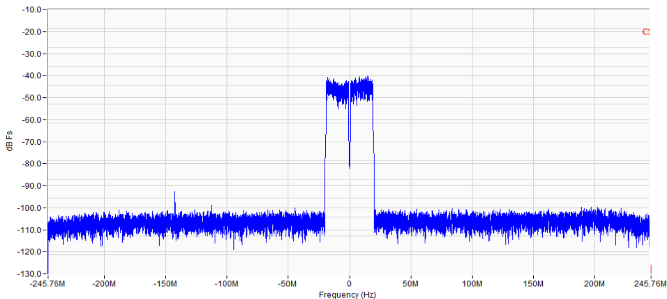
Figure 6-4. RX Output : 2x20MHz LTE signal (TX-RX Loopback) at 2.6GHz
