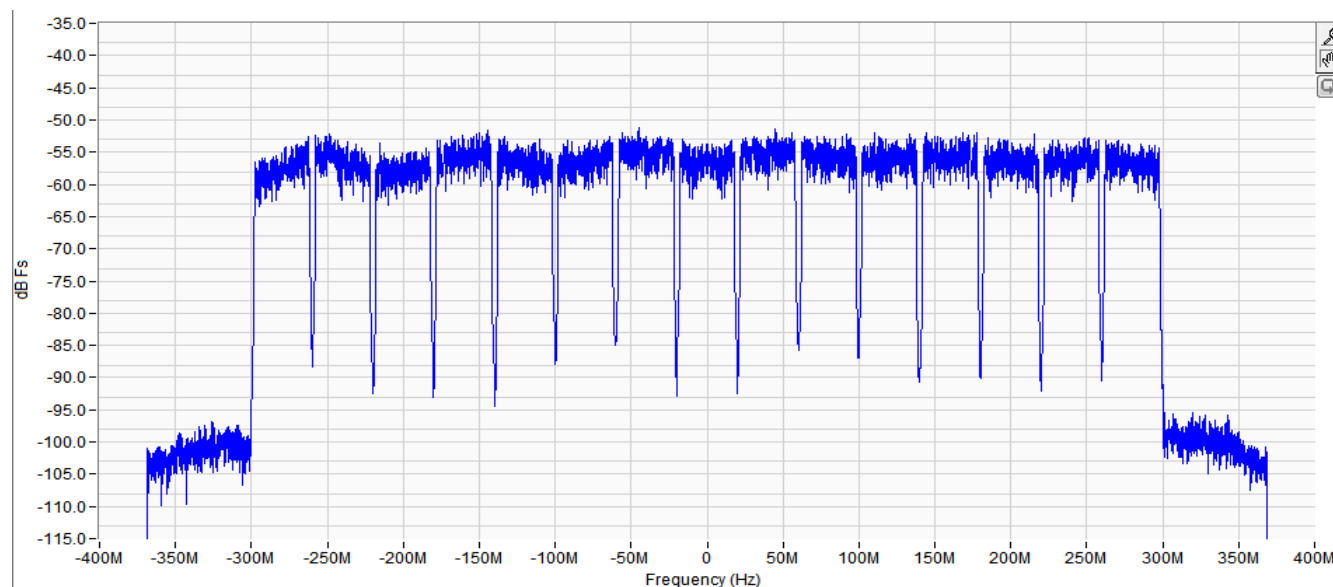
Figure 6-7. FBRX Path Output with Wideband Signal (600MHz)
