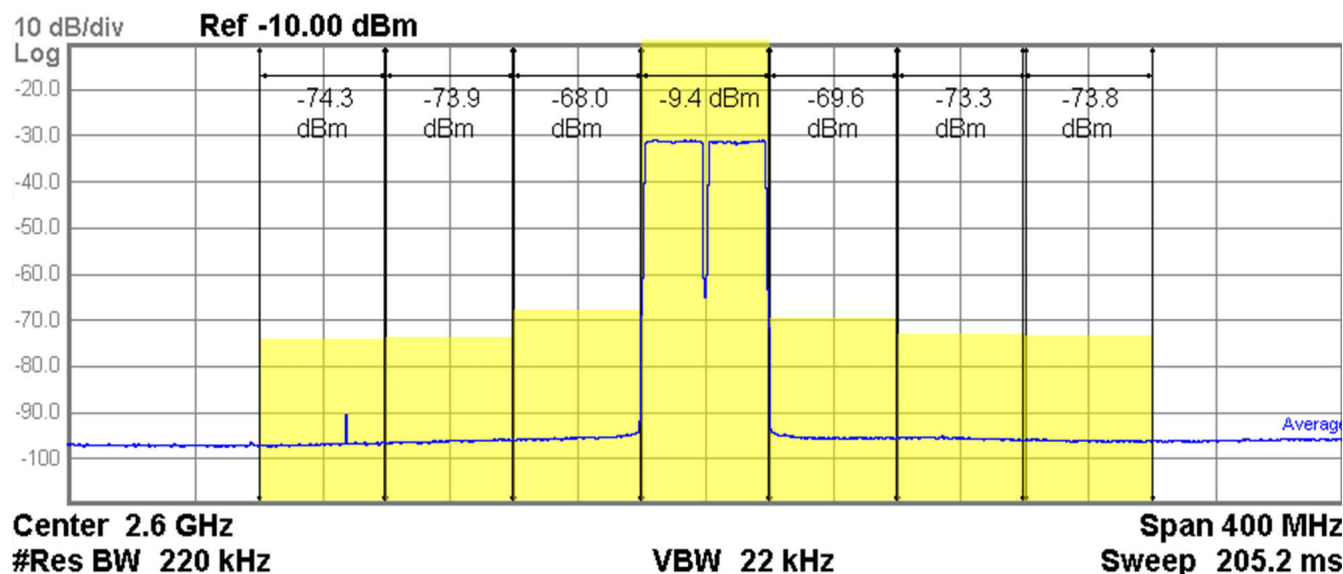
Figure 6-3. TX Output : 2x20MHz LTE Signal at 2.6GHz
