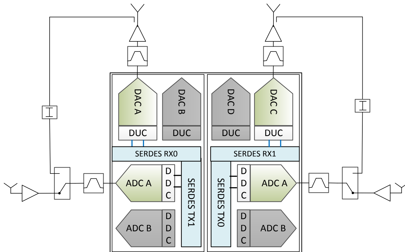
Figure 5-1. 2T2R2FB TDD Configuration
