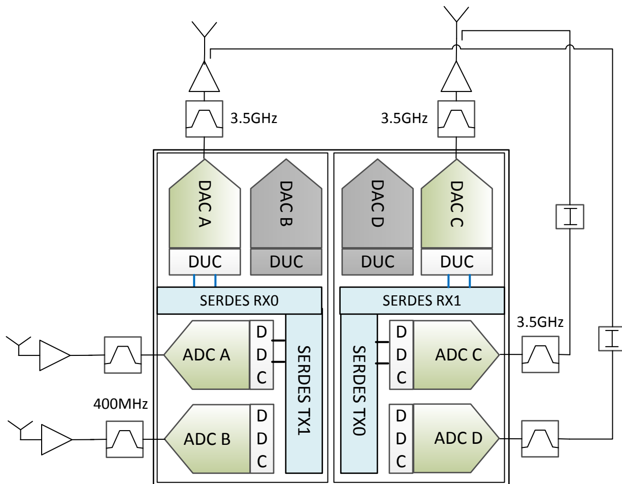
Figure 5-3. 2T2R2FB Configuration for RF Repeater
