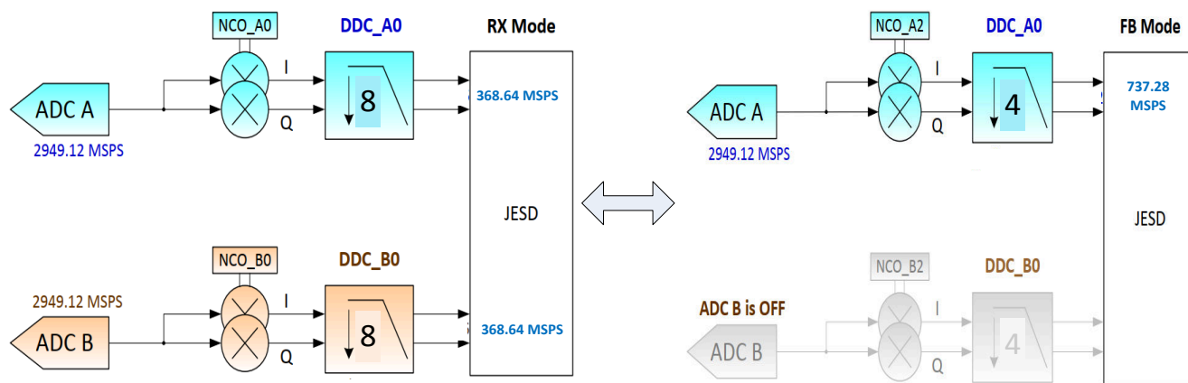
Figure 5-2. RX-to-FBRX Dynamic Switching
