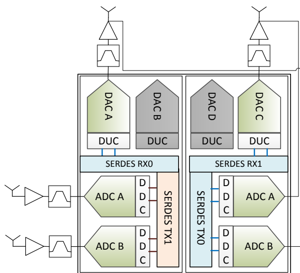
Figure 3-2. 2T2RnFB FDD Configuration
