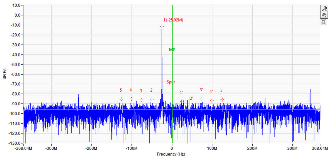
Figure 6-9. FBRX Mode Output
