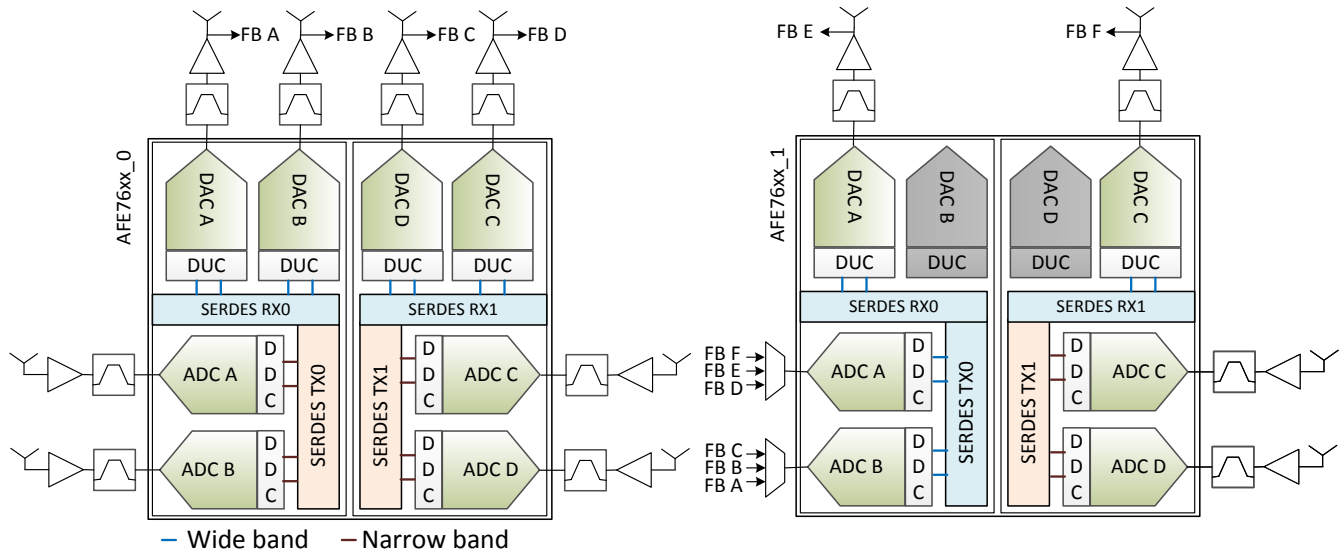
Figure 3-5. 6T6R2FB Diagram
