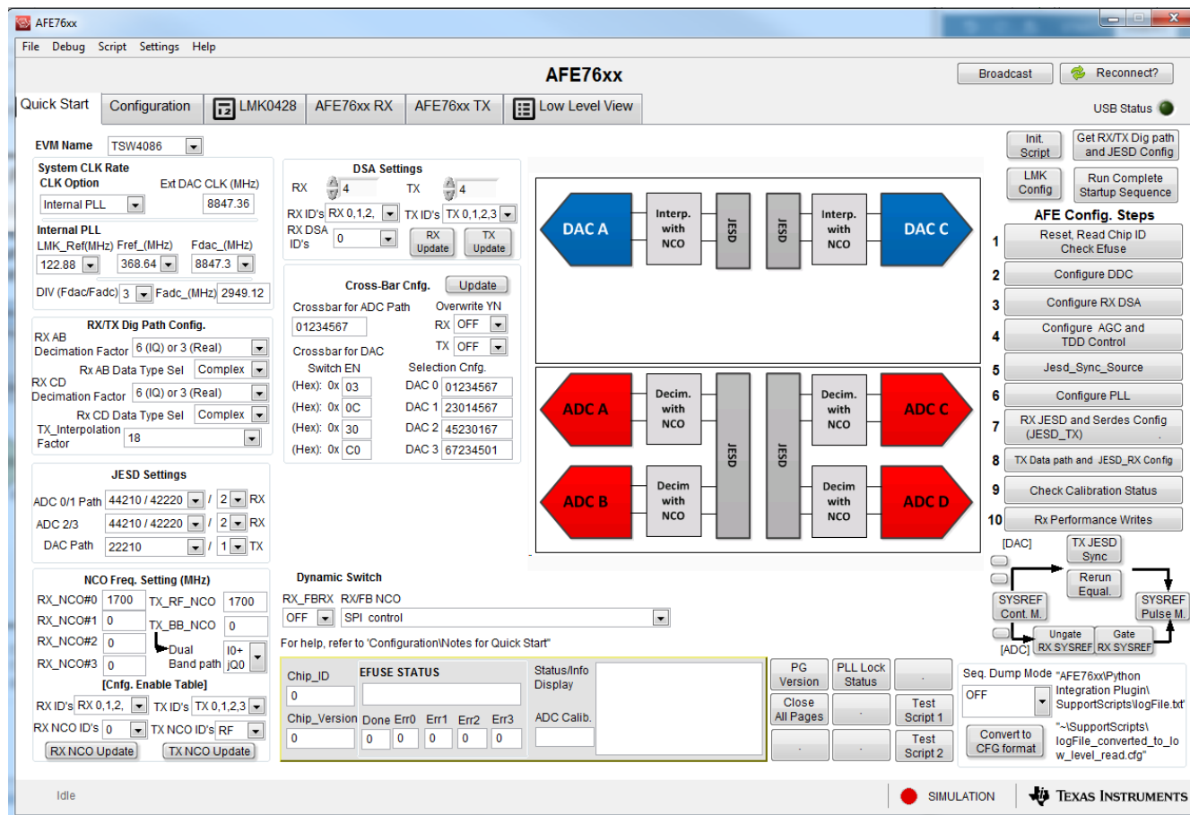
Figure 2-3. AFE76xx GUI
