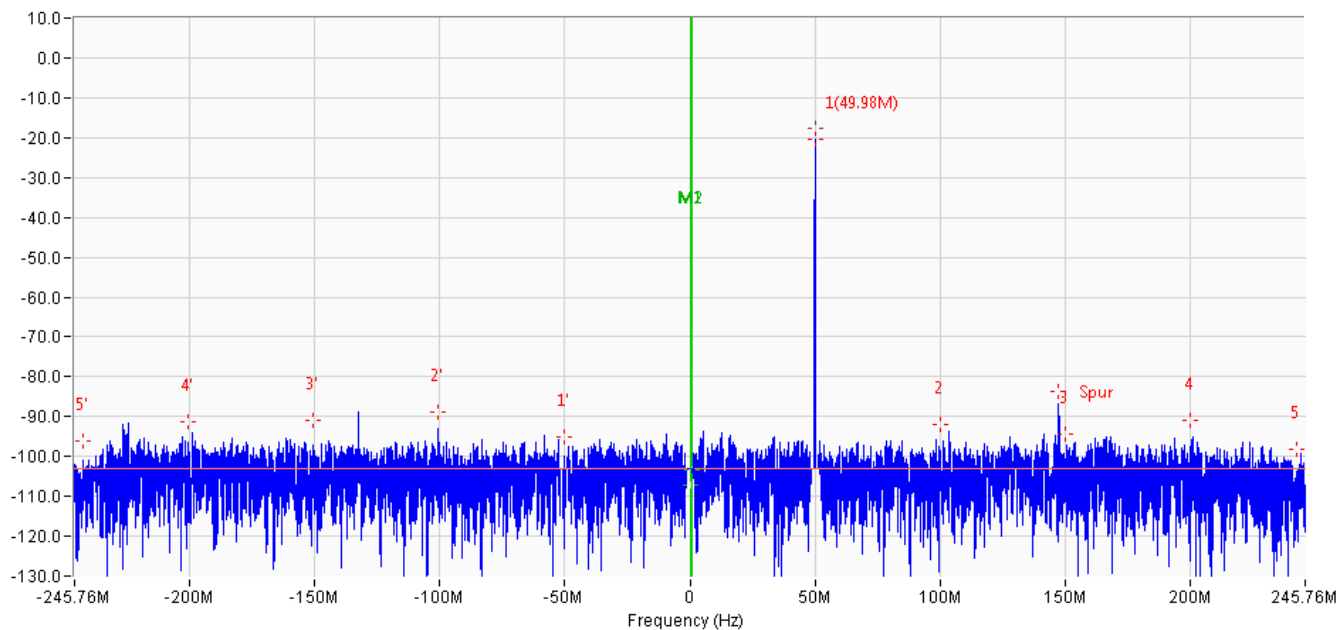
Figure 6-2. FBRX Path Output with Single Tone at 1750MHz, -15dBFS
