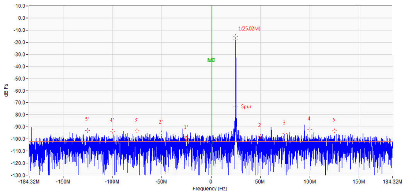
Figure 6-8. RX Mode Output
