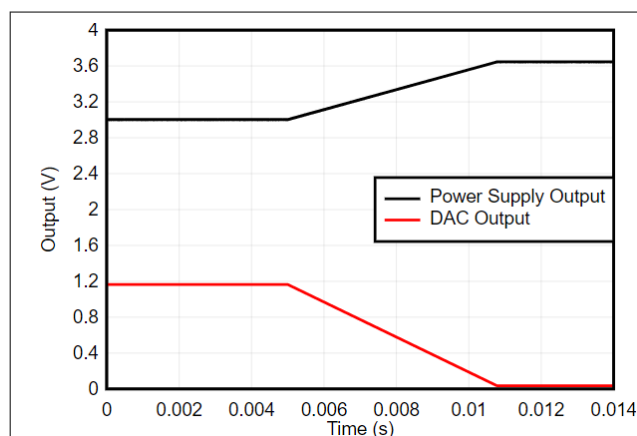
Figure 8-2. Power-Supply Margin High
