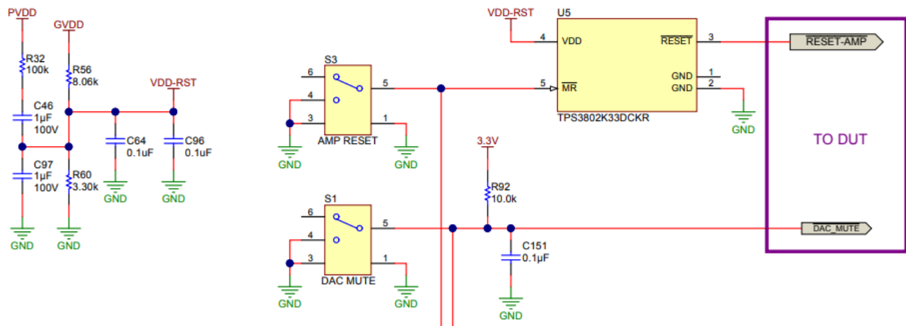
Figure 17. TAS3251EVM Reset Circuit
