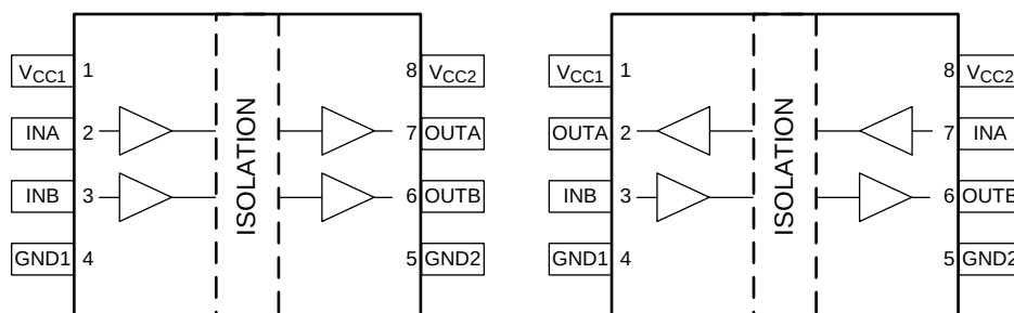
Figure 1. ISO772x Dual-Channel Digital Isolator Pin Configurations
