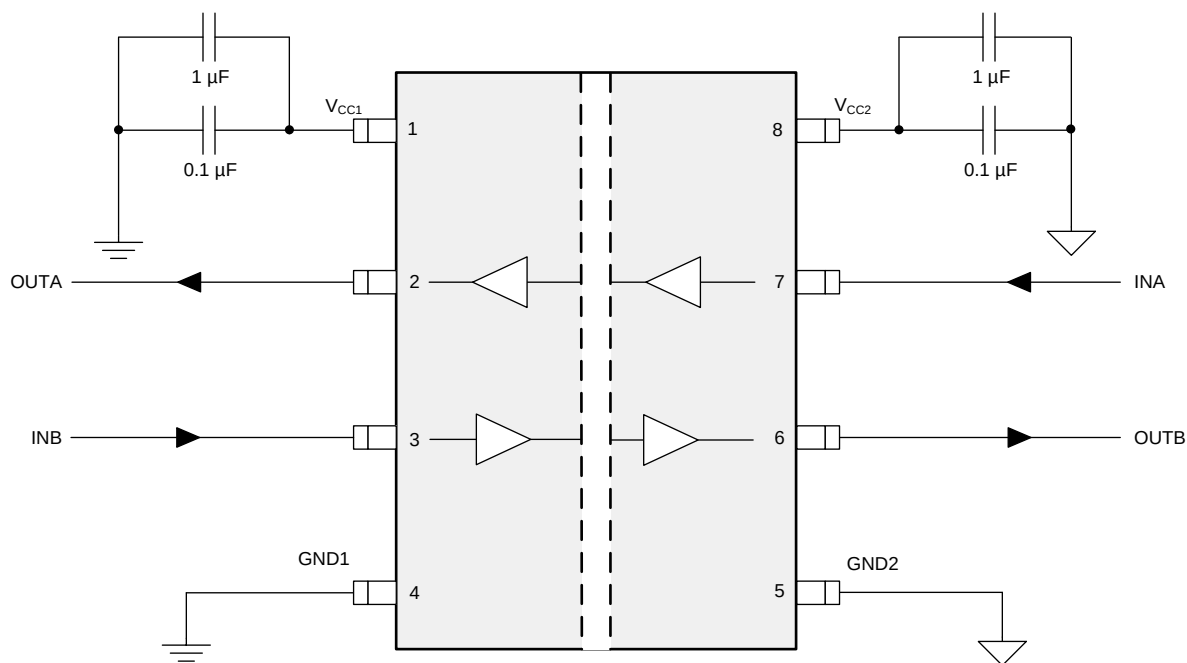
Figure 2. ISO7721 EVM Configuration
