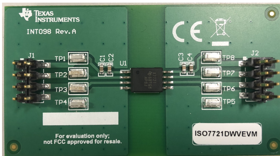
Figure 3. ISO77xxDWV-EVM Photograph
